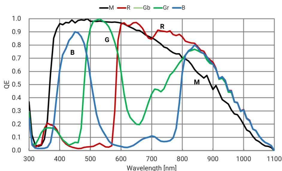
Figure 4-39 ME2C-517-23GM/C(-P) sensor spectral response
