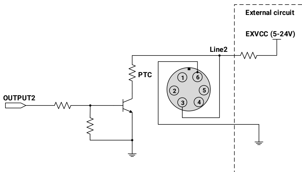
Figure 7-31 Internal equivalent circuit of camera when Line2 is configured as output (ME2S/ME2C)
