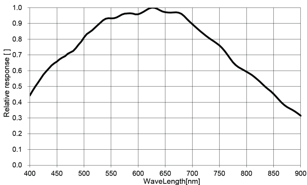
Figure 4-14 MER2-503-23GM-P POL sensor spectral response
