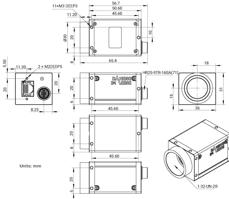
Figure 5-15 ME2P-034-491G3M-P-MS4-16P S00 mechanical dimensions
