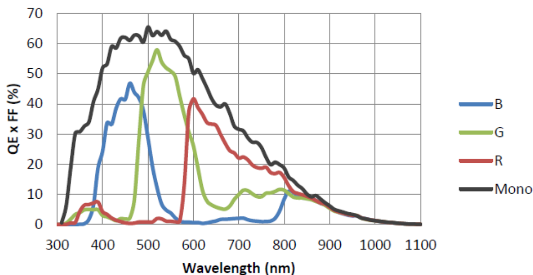
Figure 4-50 ME2P-560-21GM/C-P sensor spectral response
