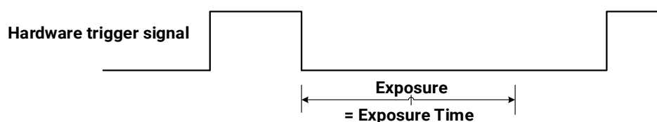
Figure 8-28 The sequence diagram in falling edge trigger of Timed exposure mode
