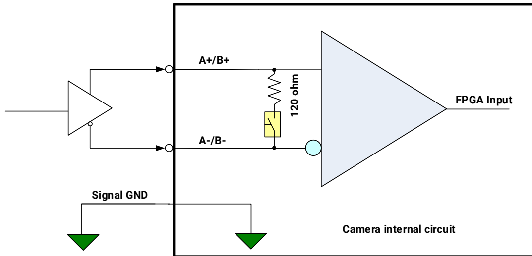
Figure 7-32 RS422 input block diagram
