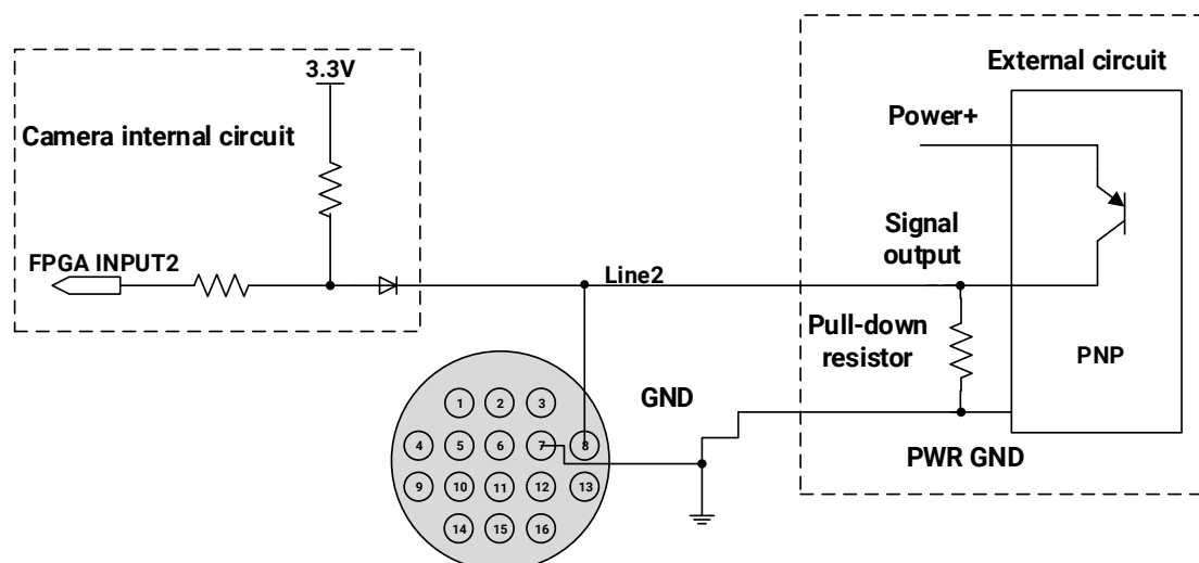
Figure 7-24 PNP photoelectric sensor connected to Line2 input circuit (ME2P Multispectral)
