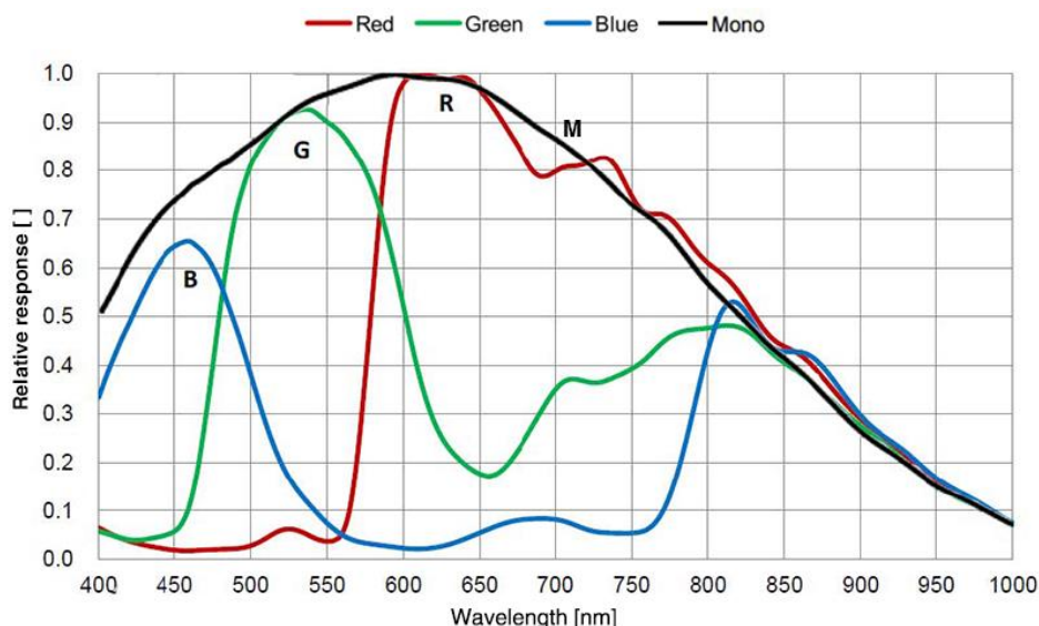
Figure 4-34 ME2C-303-37GM/C(-P) sensor spectral response
