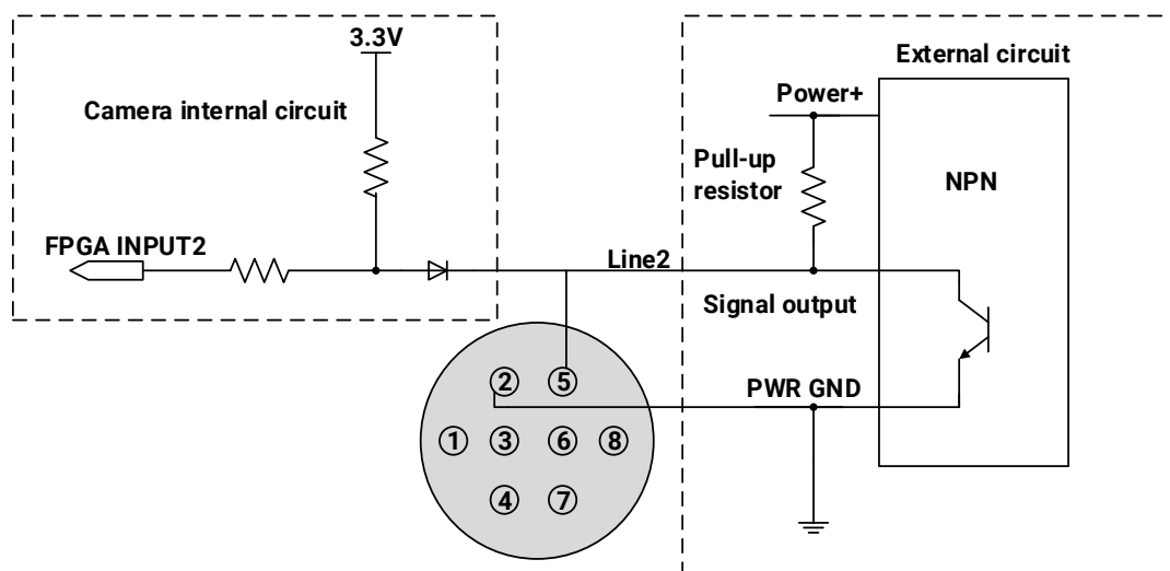
Figure 7-21 NPN photoelectric sensor connected to Line2 input circuit (MER2/ME2P)
