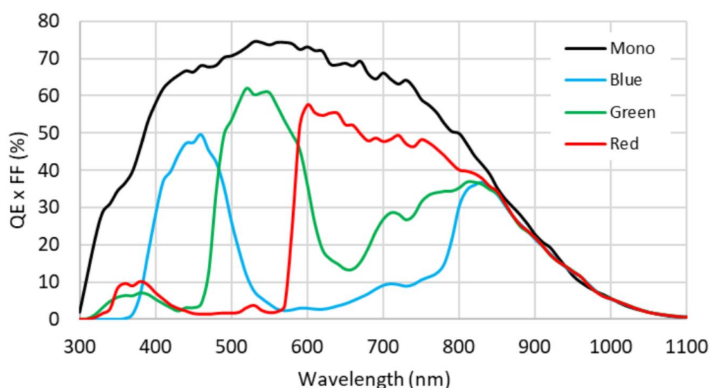
Figure 4-32 ME2C-240-48GM/C(-P) sensor spectral response
