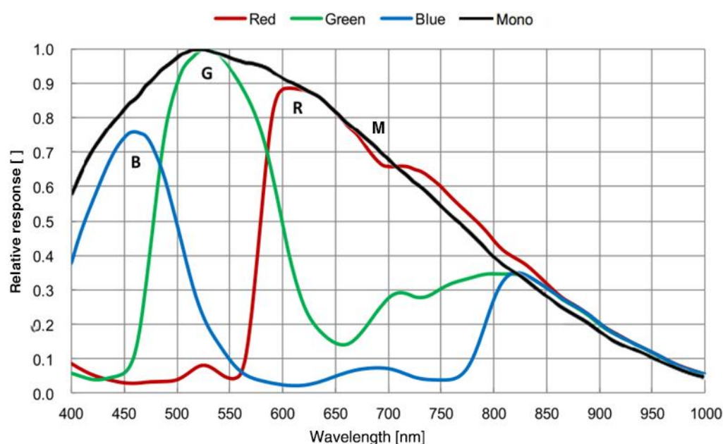
Figure 4-31 ME2C-231-41GM/C(-P) sensor spectral response
