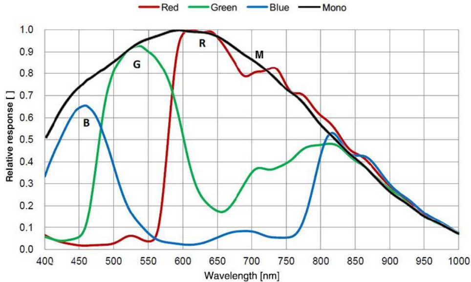
Figure 4-12 MER2-501-23GM/C(-P) sensor spectral response
