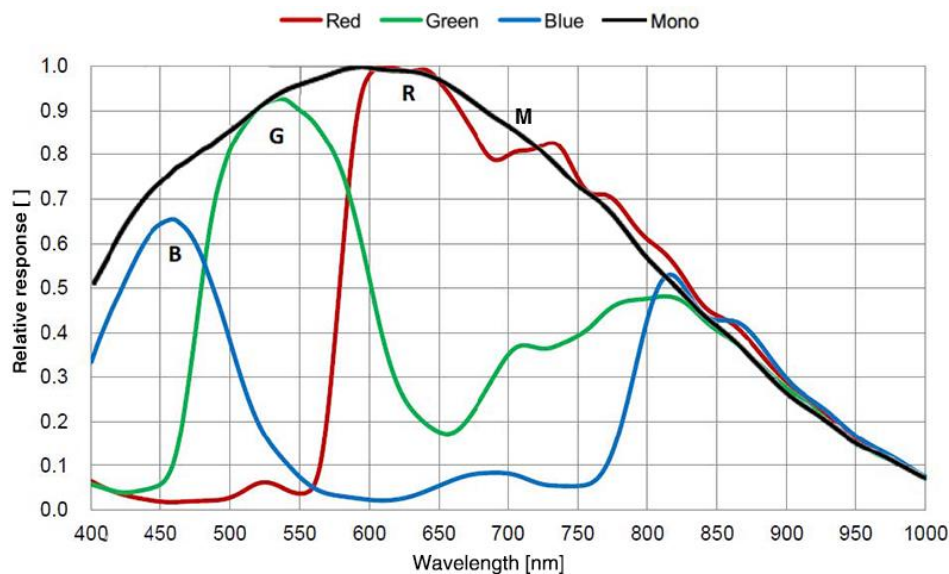
Figure 4-13 MER2-503-23GM/C(-P) sensor spectral response
