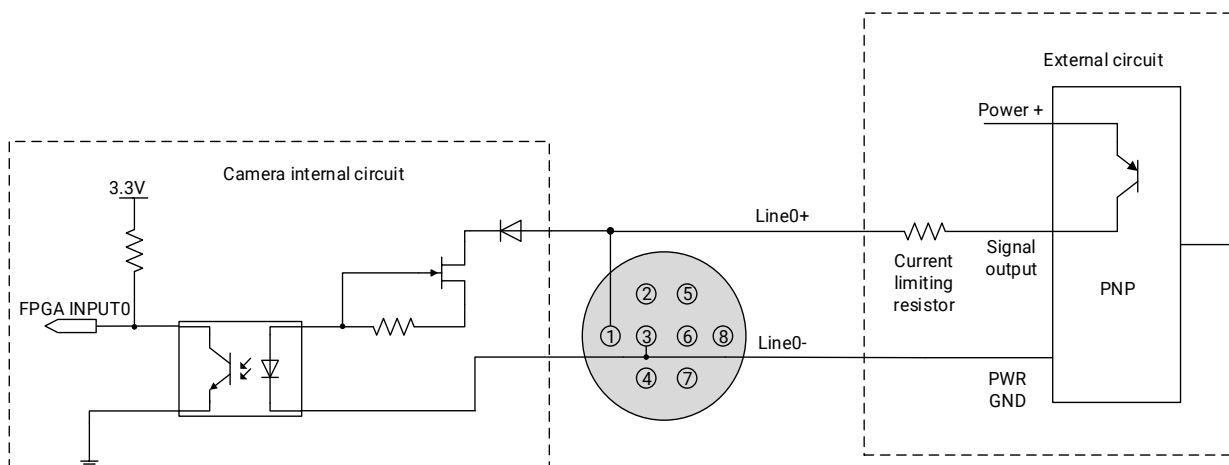
Figure 7-5 PNP photosensor connected to opto-isolated input circuit (MER2/ME2P)
