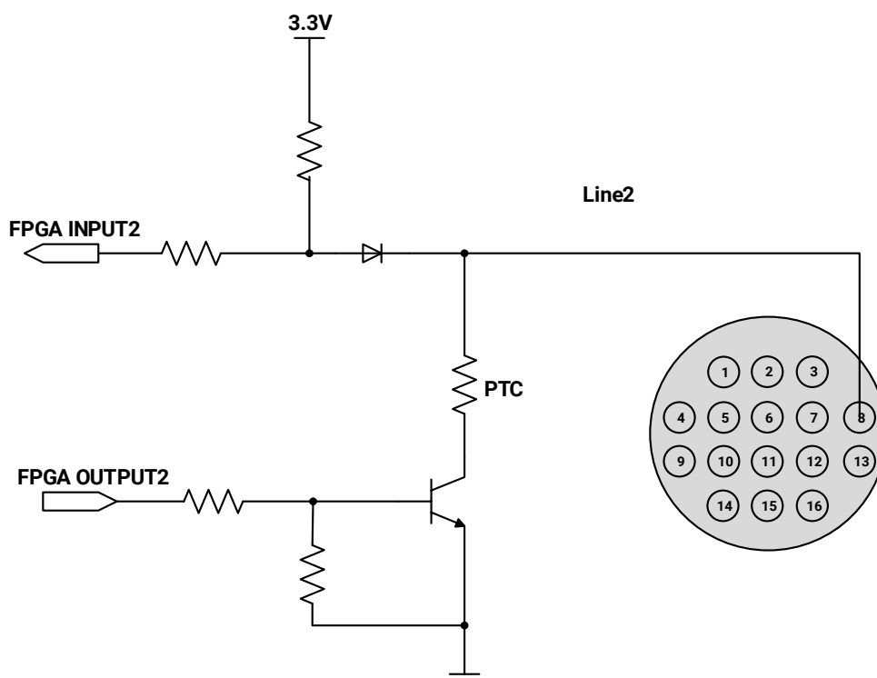
Figure 7-16 Line2/3 (bidirectional) circuit (ME2P Multispectral)
