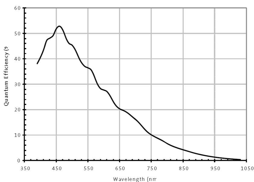
Figure 4-19 MER2-1070-10GM(-P) sensor spectral response
