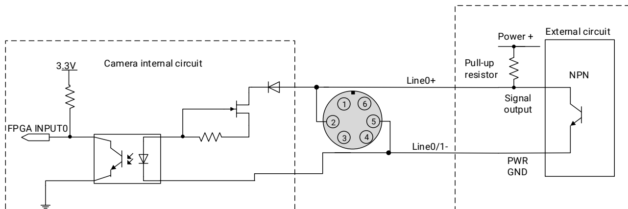
Figure 7-8 NPN photosensor connected to opto-isolated input circuit (ME2S/ME2C)
