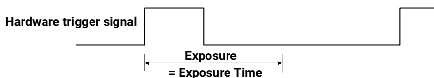
Figure 8-27 The sequence diagram in rising edge trigger of Timed exposure mode
