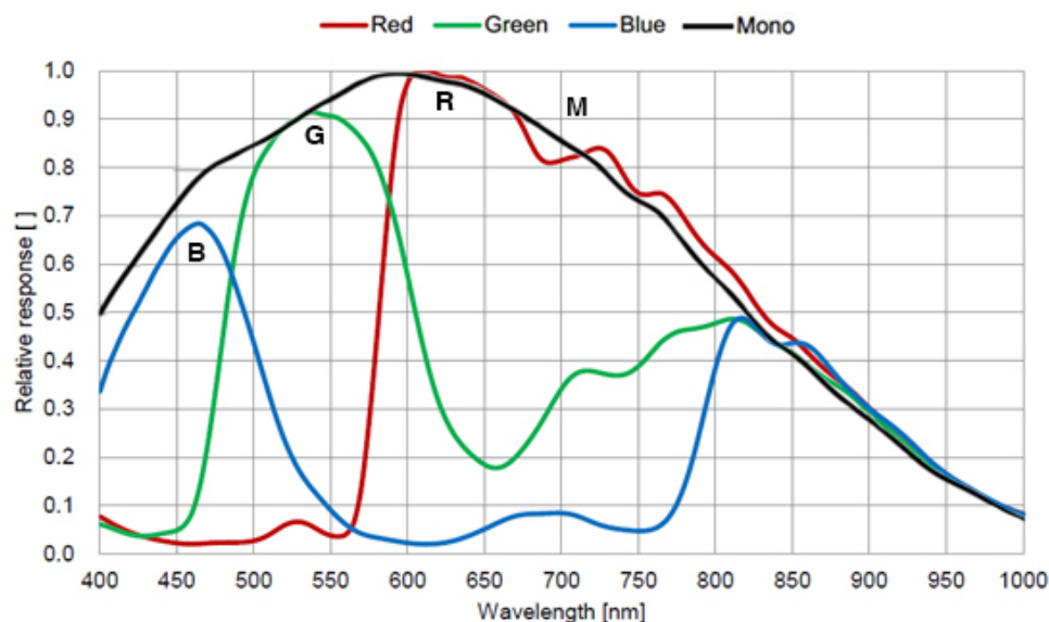
Figure 4-22 ME2C-041-302GM/C(-P) sensor spectral response
