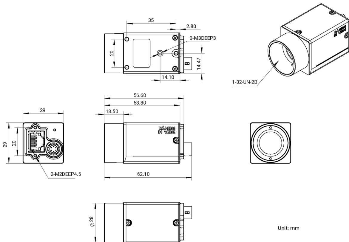
Figure 5-10 ME2C-051-120GM/C-P mechanical dimensions
