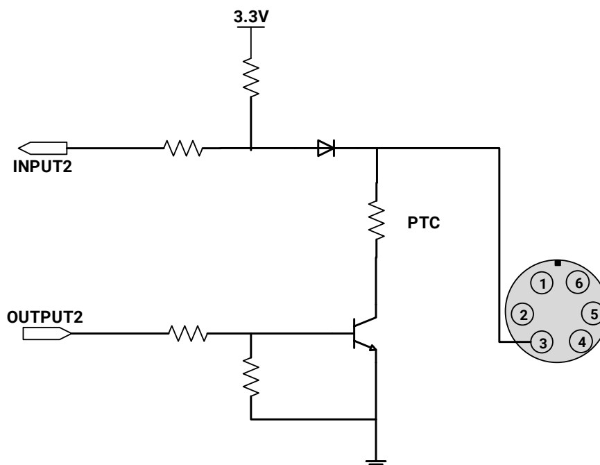
Figure 7-17 Line2 (bidirectional) circuit (ME2S/ME2C)
