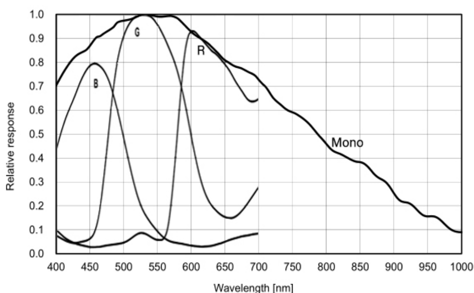
Figure 4-21 MER2-2000-6GM/C(-P) sensor spectral response
