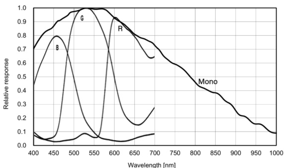
Figure 4-45 ME2C-2001-6GM(-P) sensor spectral response
