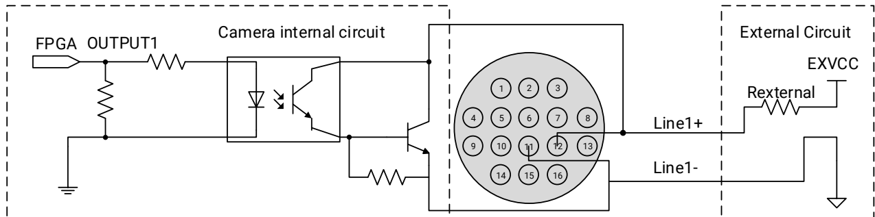
Figure 7-12 Opto-isolated output circuit (ME2P Multispectral)
