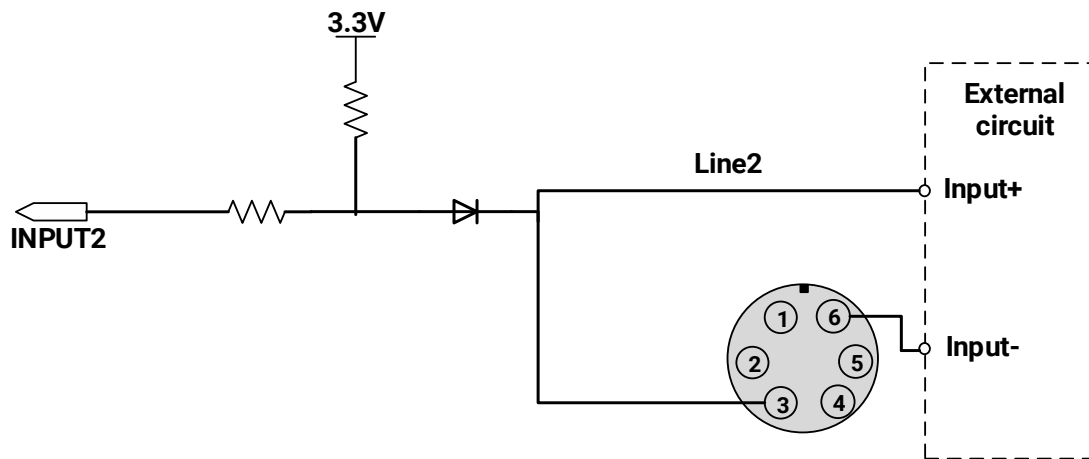
Figure 7-20 Internal equivalent circuit of camera when Line2 is configured as input (ME2S/ME2C)
