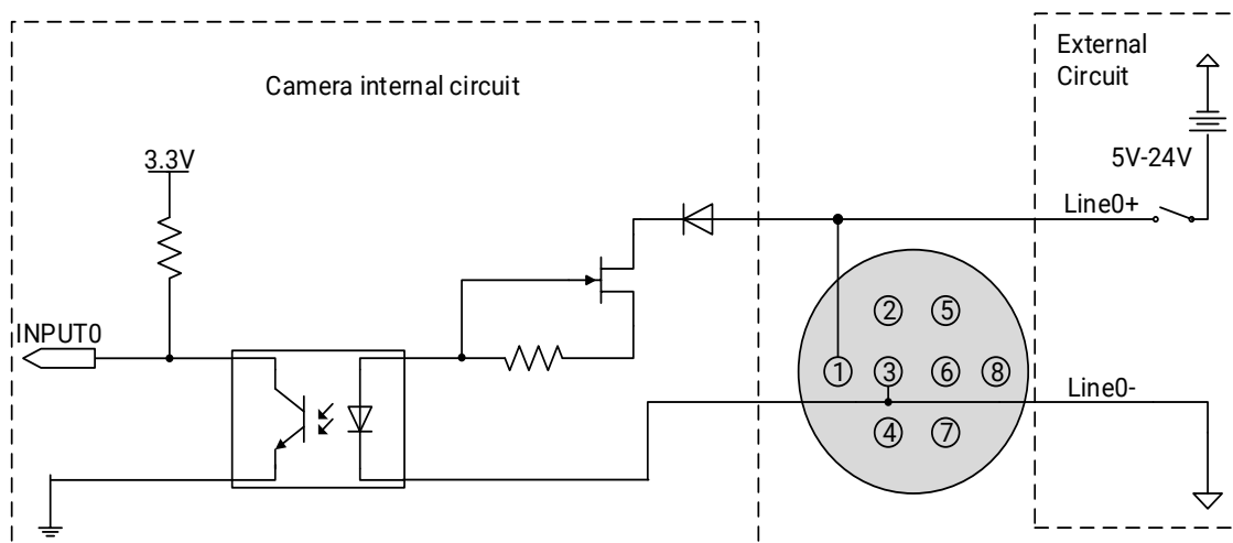
Figure 7-1 Opto-isolated input circuit (MER2/ME2P)
