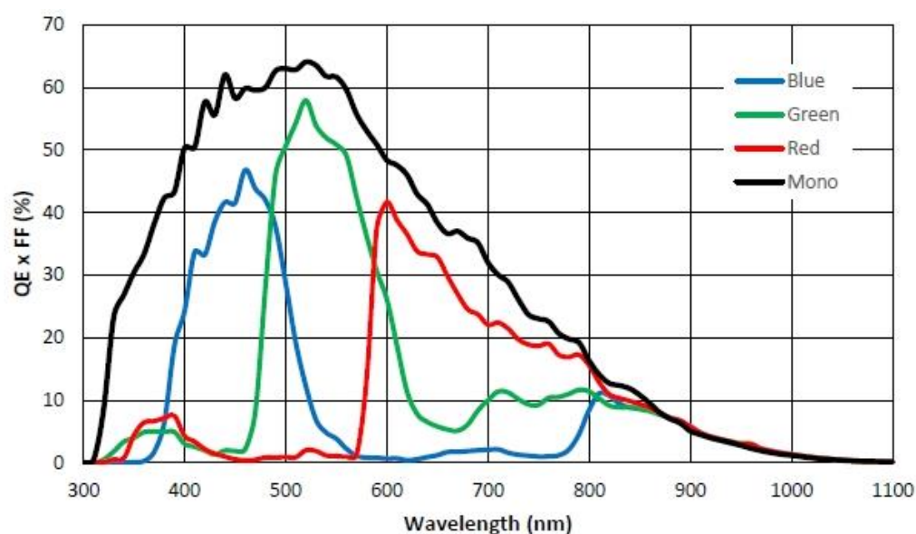
Figure 4-53 ME2P-1840-6GM/C-P \ ME2P-1842-6GC-P sensor spectral response
