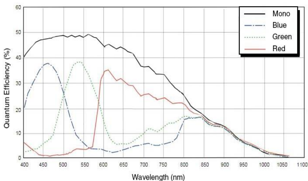
Figure 4-28 ME2C-202-60GM/C(-P) sensor spectral response
