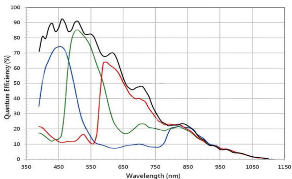
Figure 4-37 ME2C-507-23GM/C(-P) sensor spectral response
