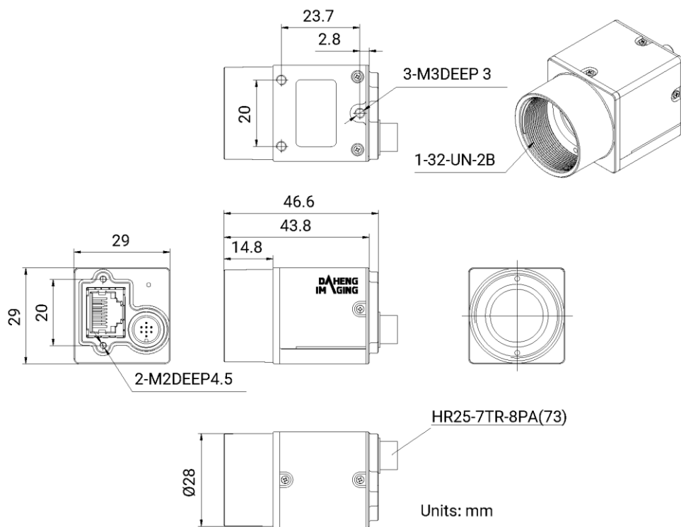
Figure 5-5 MER2-532-22GM/C mechanical dimensions
