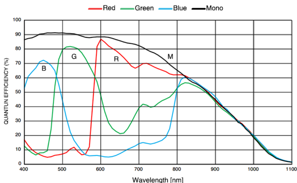
Figure 4-46 ME2C-2002-6GM/C sensor spectral response
