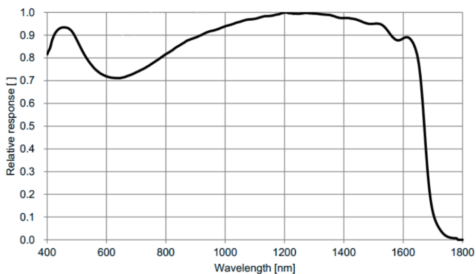
Figure 4-59 ME2P-034-491G3M-P-MS4-16P S00 sensor spectral response
