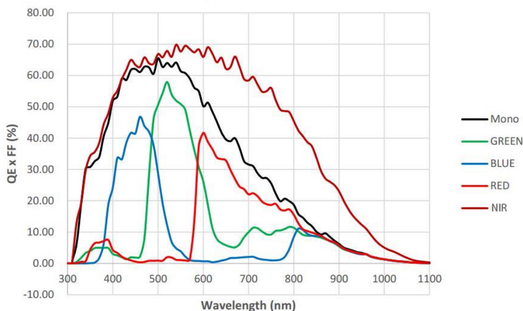
Figure 4-54 ME2P-2621-4GM/C-P \ ME2P-2622-4GM/C-P sensor spectral response
