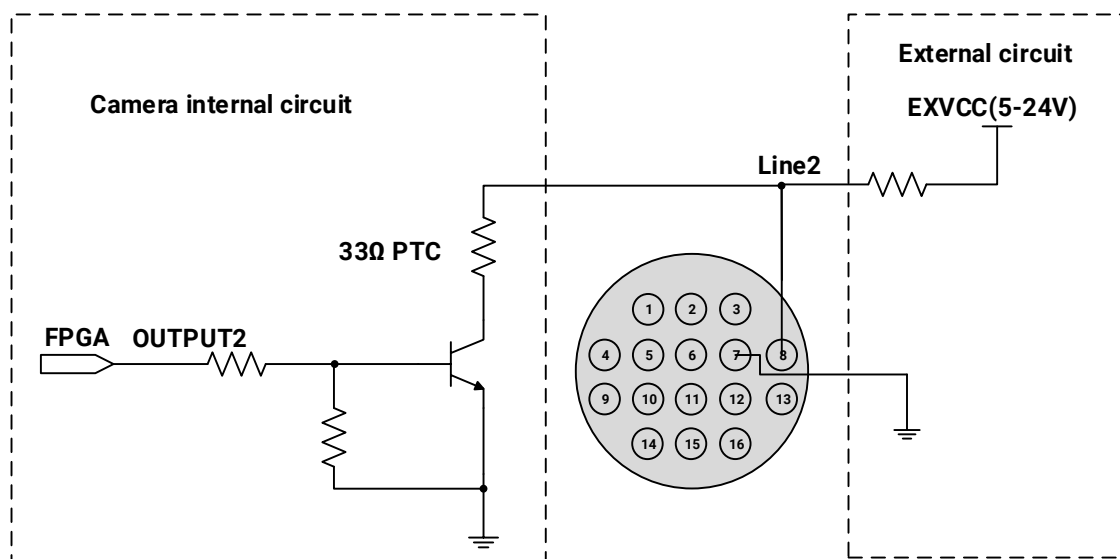
Figure 7-30 Internal equivalent circuit of camera when Line2 is configured as output (ME2P Multispectral)
