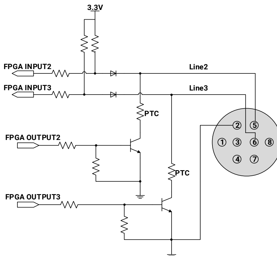
Figure 7-15 Line2/3 (bidirectional) circuit (MER2/ME2P)
