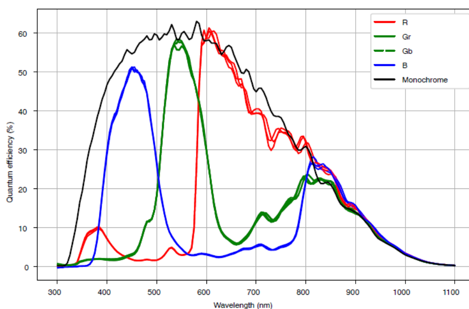
Figure 4-17 MER2-532-22GM/C sensor spectral response
