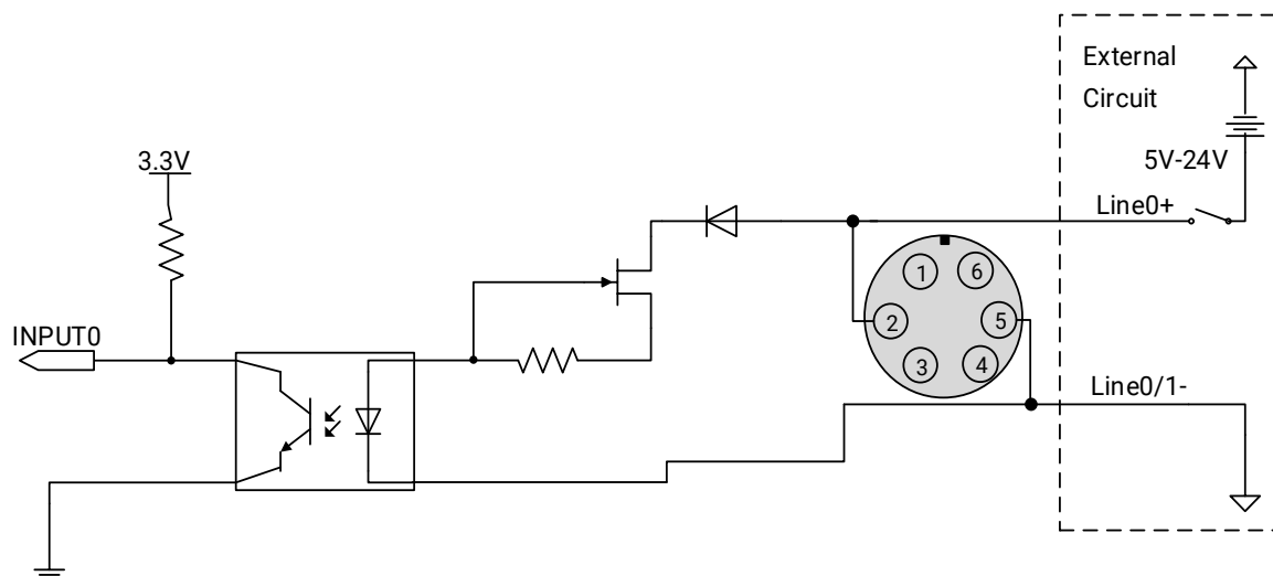
Figure 7-3 Opto-isolated input circuit (ME2S/ME2C)
