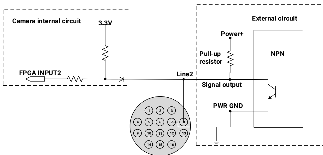
Figure 7-23 NPN photoelectric sensor connected to Line2 input circuit (ME2P Multispectral)
