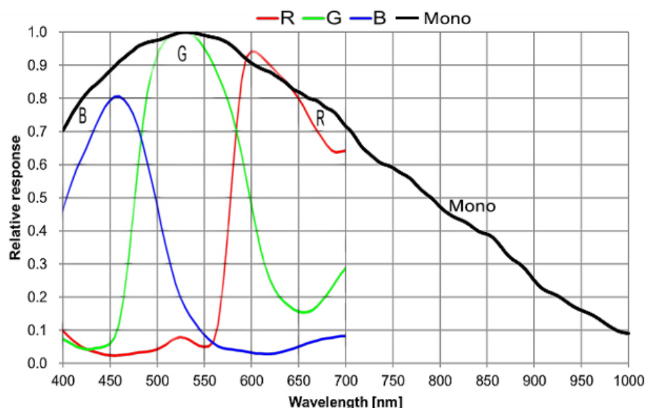
Figure 4-18 MER2-630-18GM/C(-P/-W90-S90) sensor spectral response
