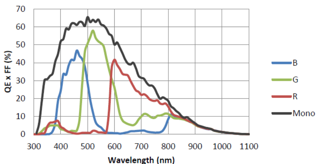
Figure 4-51 ME2P-900-13GM/C-P sensor spectral response
