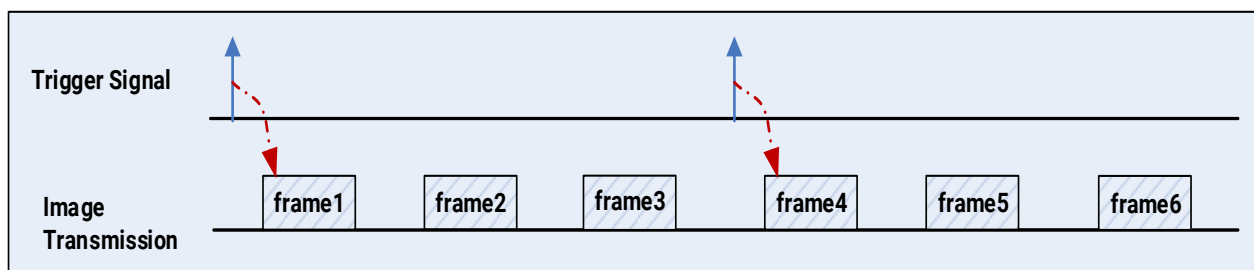
Figure 8-19 FrameBurstStart trigger
