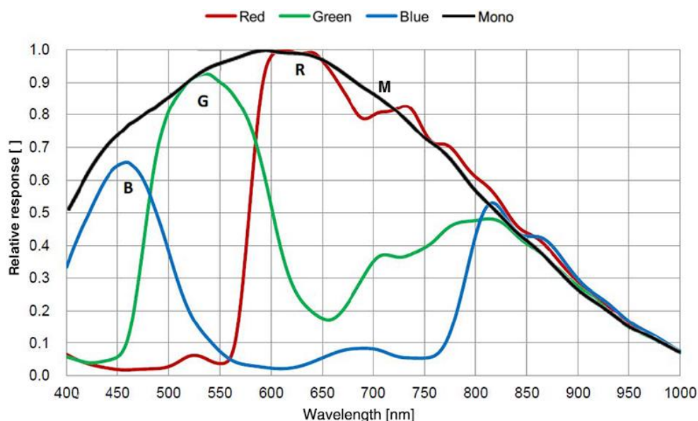
Figure 4-35 ME2C-501-23GM/C(-P) sensor spectral response
