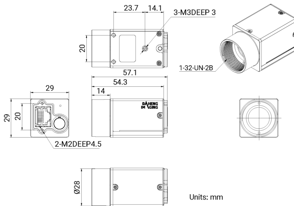
Figure 5-3 MER2 -G-P-L mechanical dimensions
