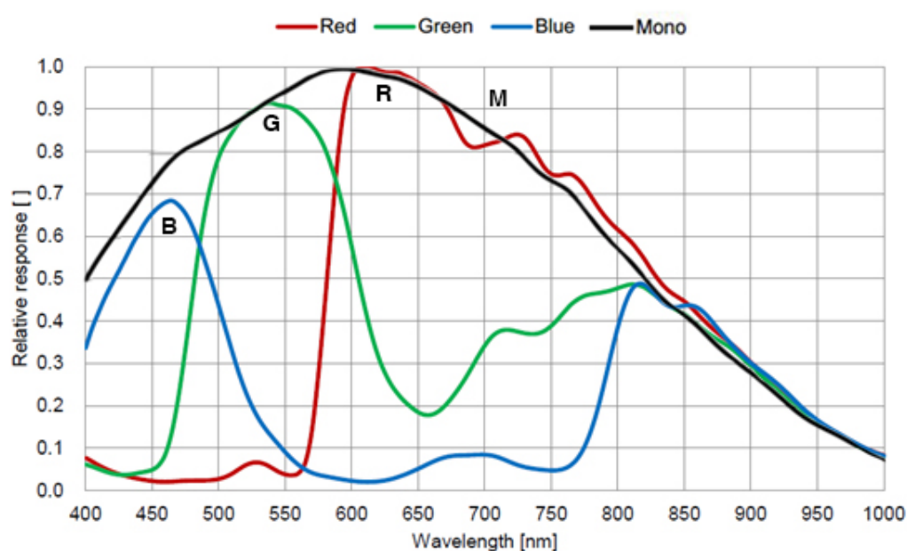
Figure 4-1 MER2-041-302GM/C(-P) sensor spectral response
