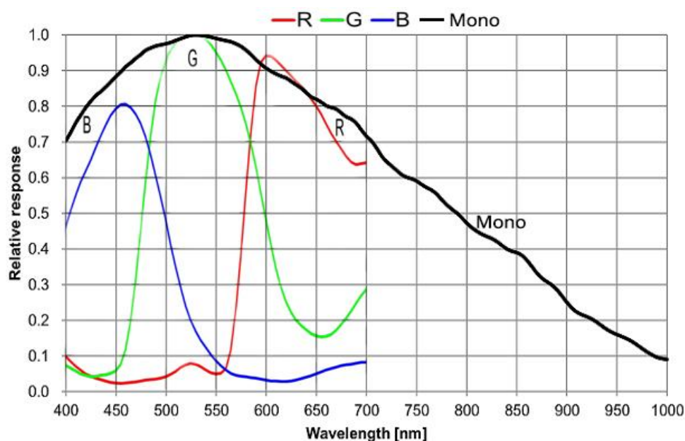
Figure 4-41 ME2C-630-18GM/C(-P) sensor spectral response
