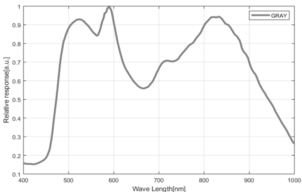
Figure 4-29 ME2C-203-30GC-P-L sensor spectral response
