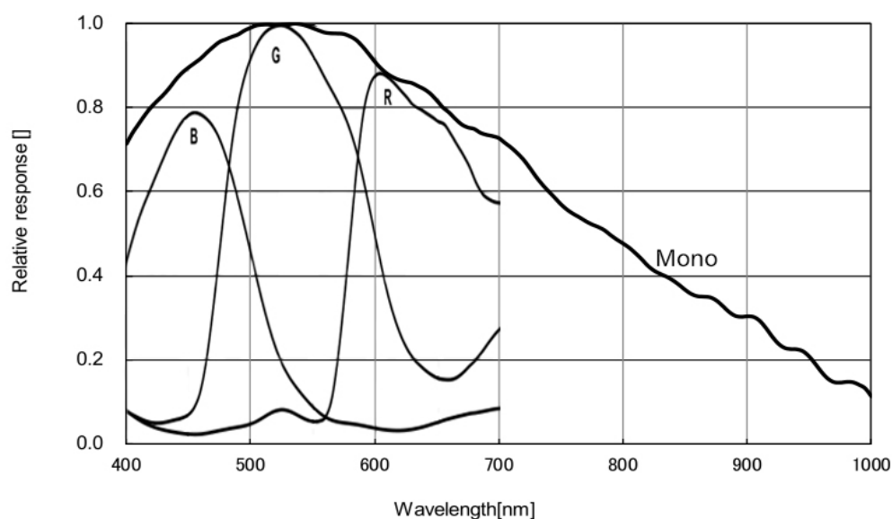
Figure 4-20 MER2-1220-9GM/C(-P) sensor spectral response
