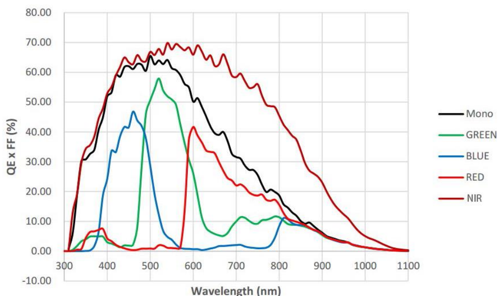
Figure 4-58 ME2P-2621-4GM-P NIR \ ME2P-2622-4GM-P NIR sensor spectral response
