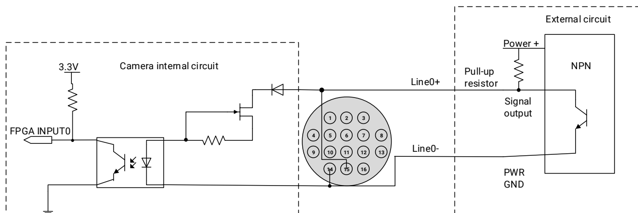
Figure 7-6 NPN photosensor connected to opto-isolated input circuit (ME2P Multispectral)
