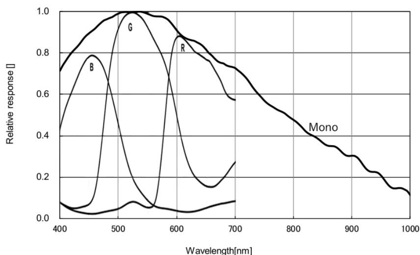
Figure 4-43 ME2C-1220-9GM/C(-P) sensor spectral response
