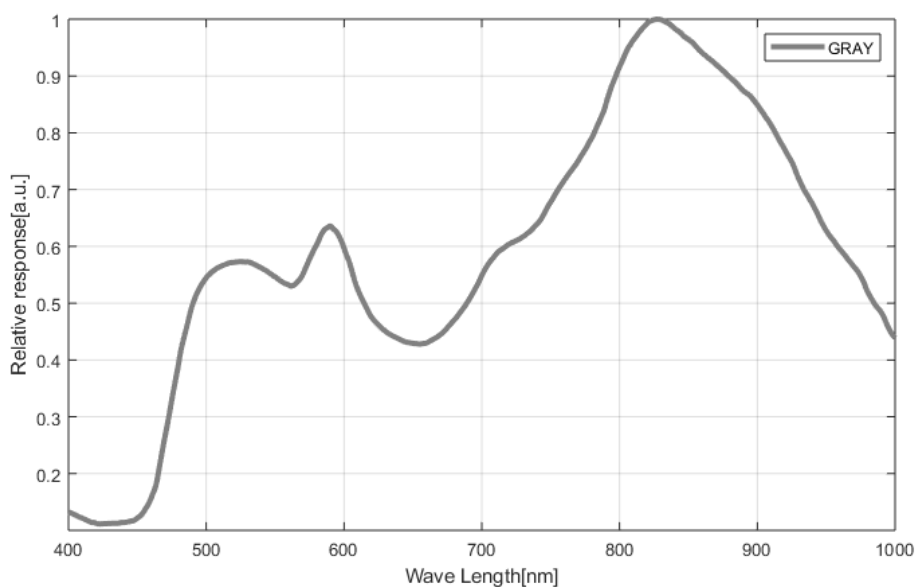
Figure 4-30 ME2C-204-30GC-P-L sensor spectral response
