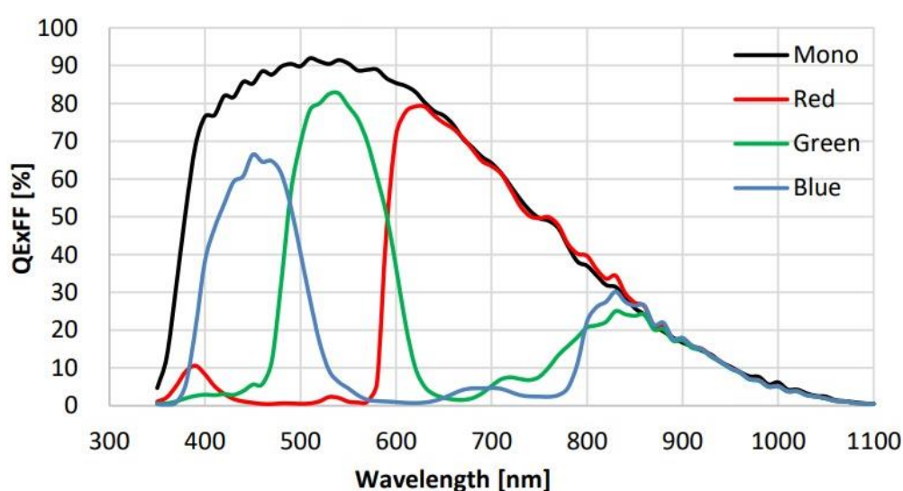
Figure 4-47 ME2C-2460-4GM/C sensor spectral response
