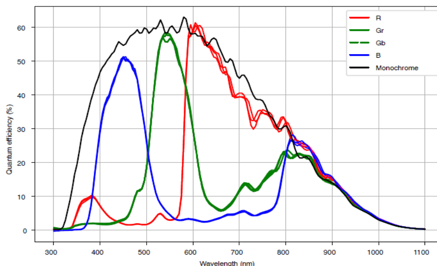
Figure 4-48 ME2S-1260-9GM/C-P sensor spectral response
