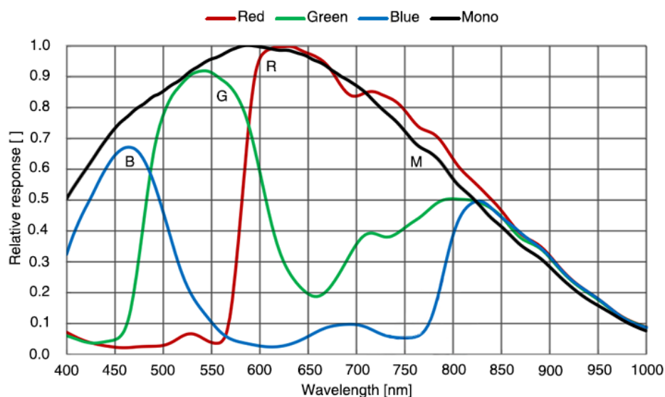
Figure 4-49 ME2P-171-66GM/C-P sensor spectral response
