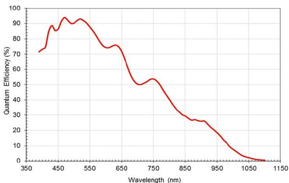
Figure 4-38 ME2C-507-23GM(-P) NIR sensor spectral response
