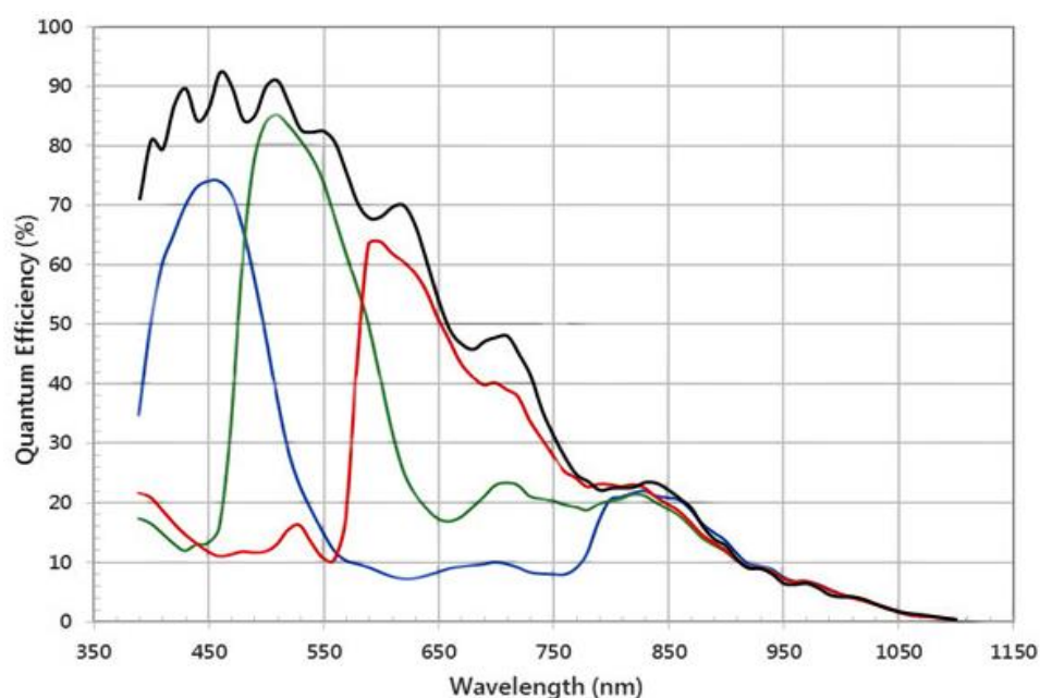
Figure 4-15 MER2-507-23GM/C(-P) sensor spectral response
