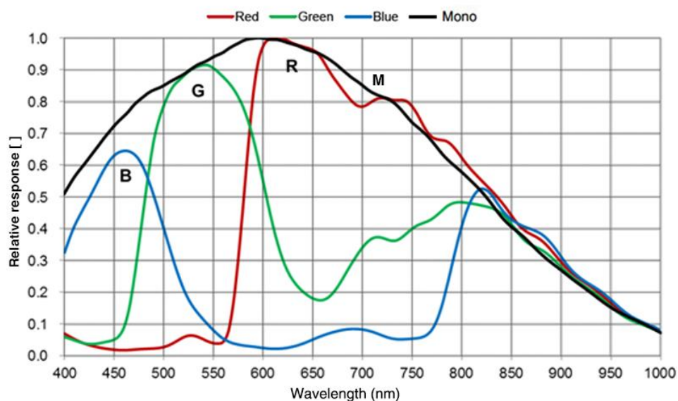
Figure 4-52 ME2P-1230-9GM/C-P sensor spectral response
