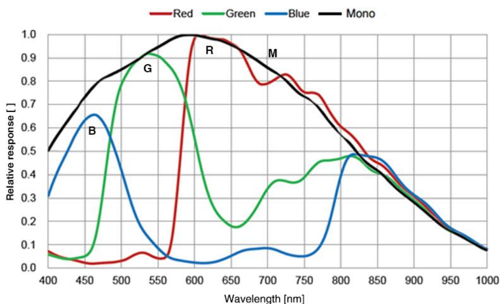
Figure 4-5 MER2-160-75GM/C(-P) sensor spectral response
