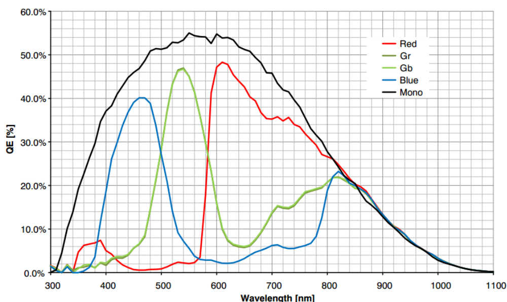
Figure 4-24 ME2C-051-120GM/C(-P) sensor spectral response
