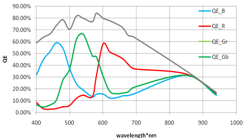
Figure 4-25 ME2C-137-90GM/C(-P) sensor spectral response
