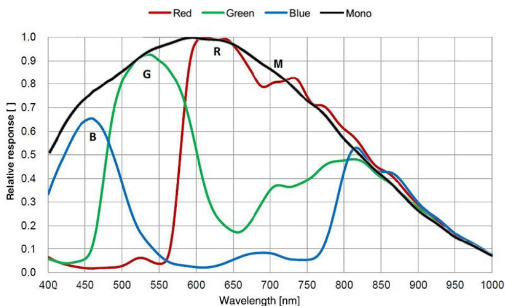
Figure 4-33 ME2C-302-37GM/C(-P) sensor spectral response
