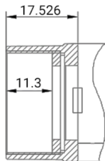
Figure 5-16 Optical interface of C-mount
