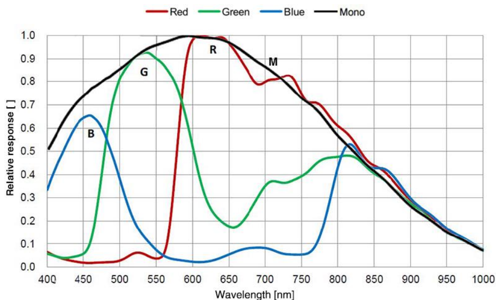
Figure 4-36 ME2C-503-23GM/C(-P) sensor spectral response
