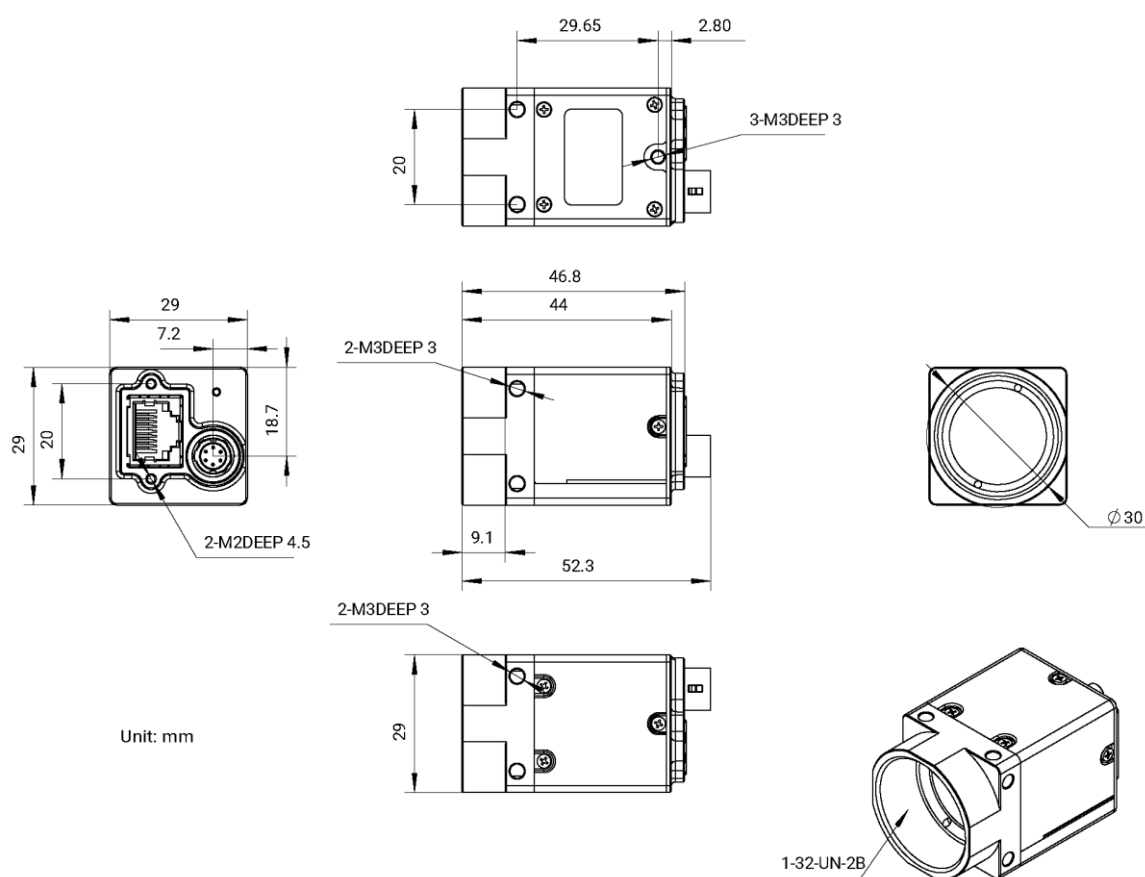
Figure 5-12 ME2C-2460-4GM/C mechanical dimensions
