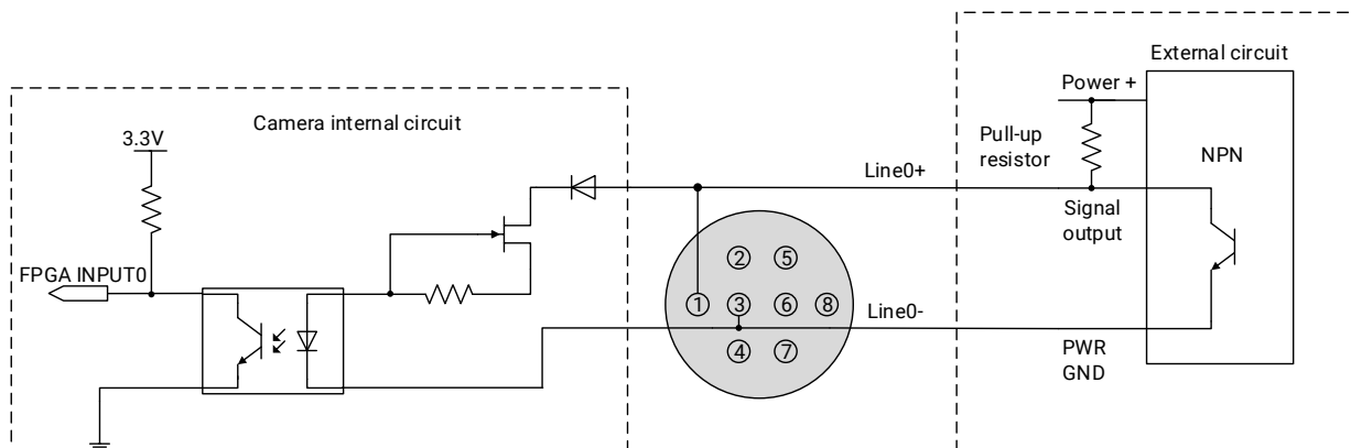
Figure 7-4 NPN photosensor connected to opto-isolated input circuit (MER2/ME2P)
