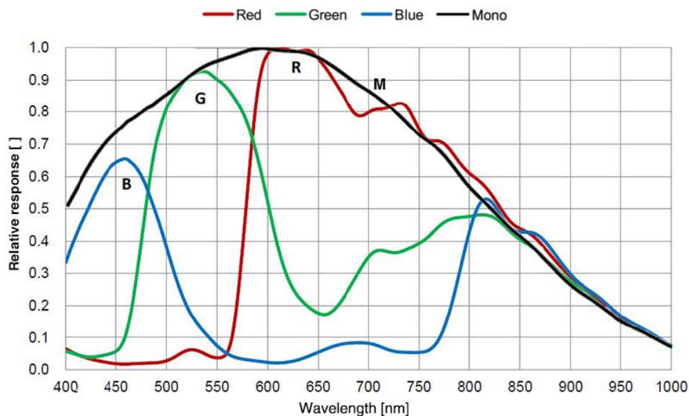
Figure 4-10 MER2-302-37GM/C(-P) sensor spectral response
