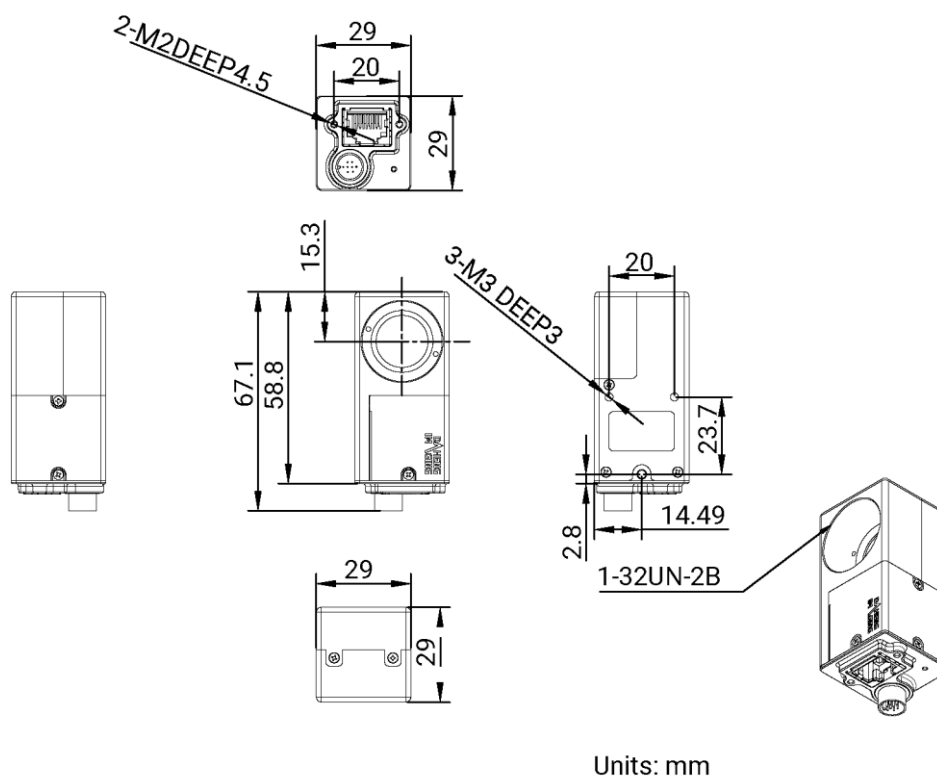
Figure 5-4 MER2-G-W90-S90 mechanical dimensions
