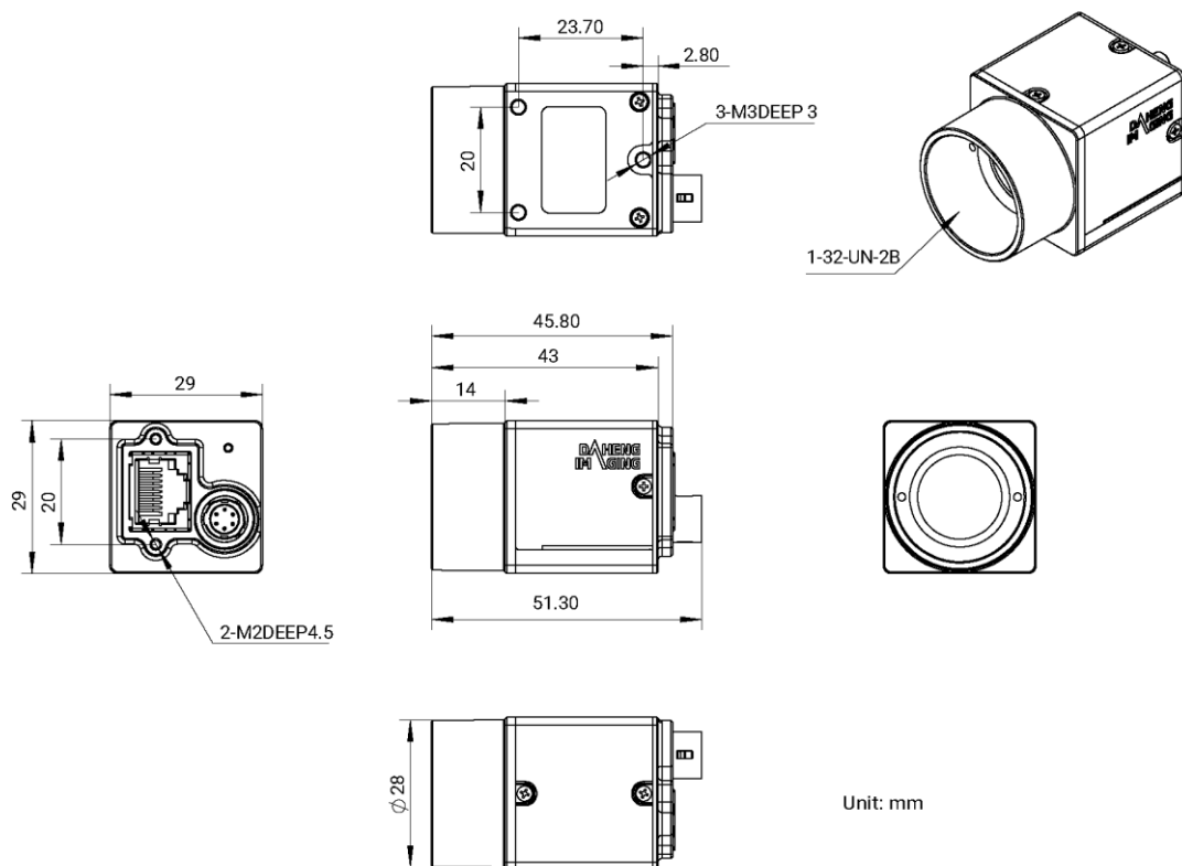
Figure 5-6 ME2C-G mechanical dimensions
