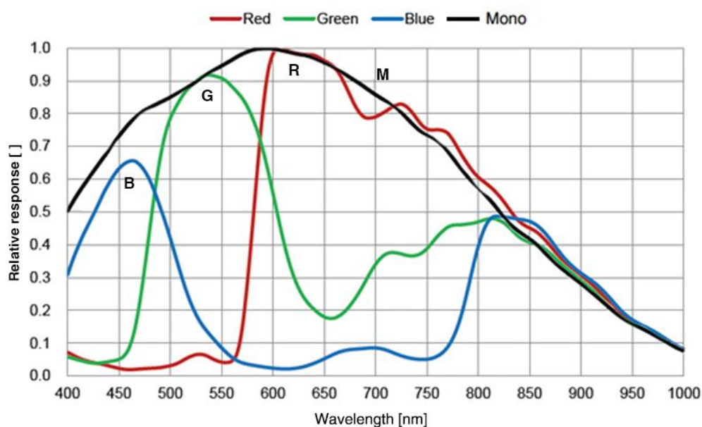
Figure 4-27 ME2C-161-75GM/C sensor spectral response
