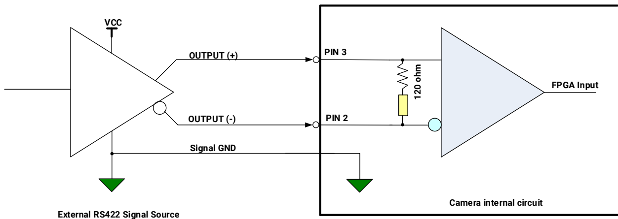
Figure 7-33 RS422 input wiring diagram
