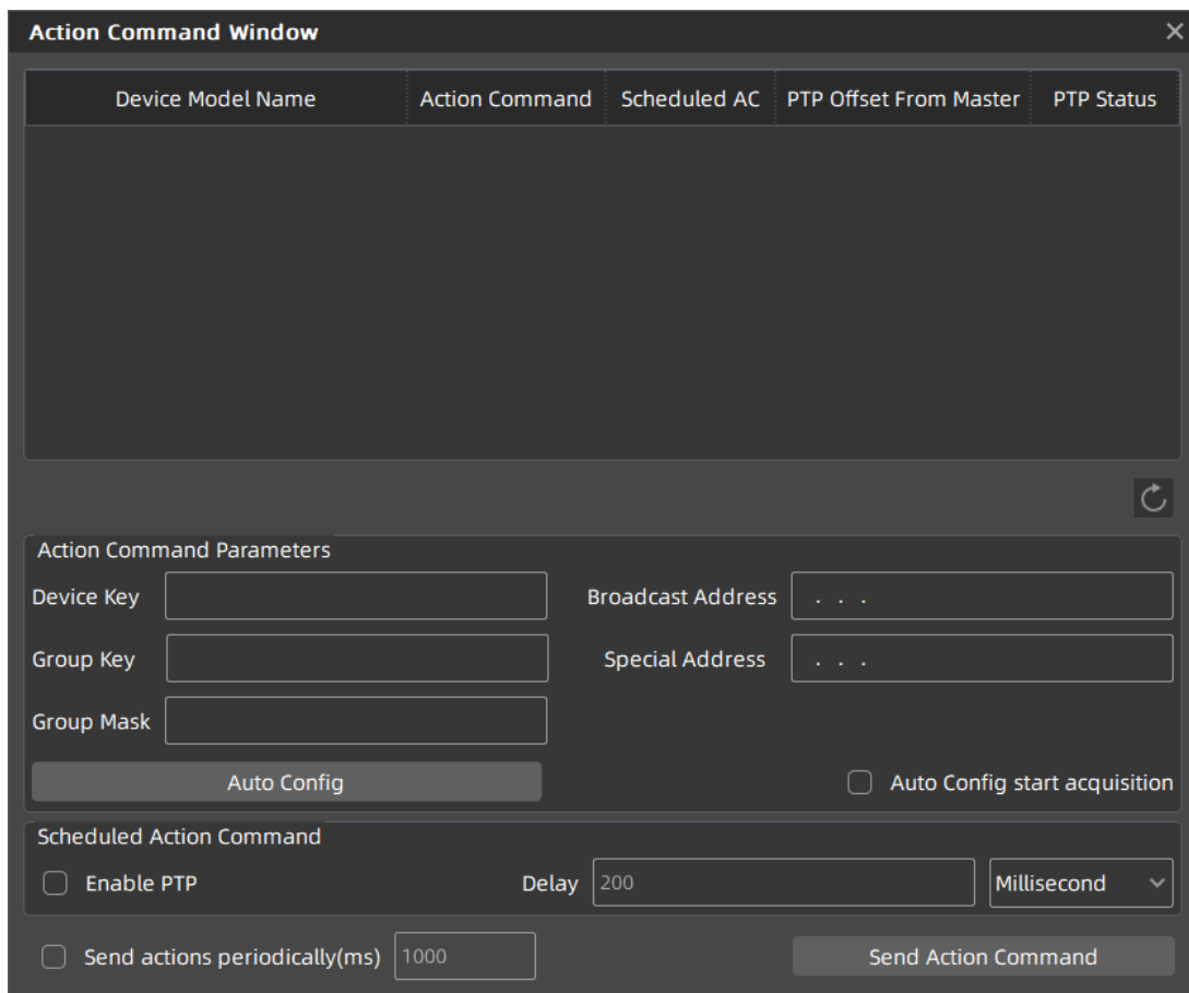
Figure 9-15 Action command window
