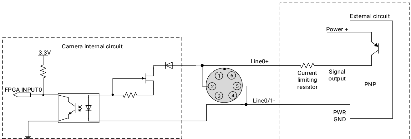
Figure 7-9 PNP photosensor connected to opto-isolated input circuit (ME2S/ME2C)
