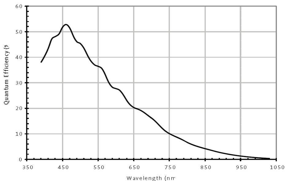
Figure 4-42 ME2C-1070-10GM(-P) sensor spectral response
