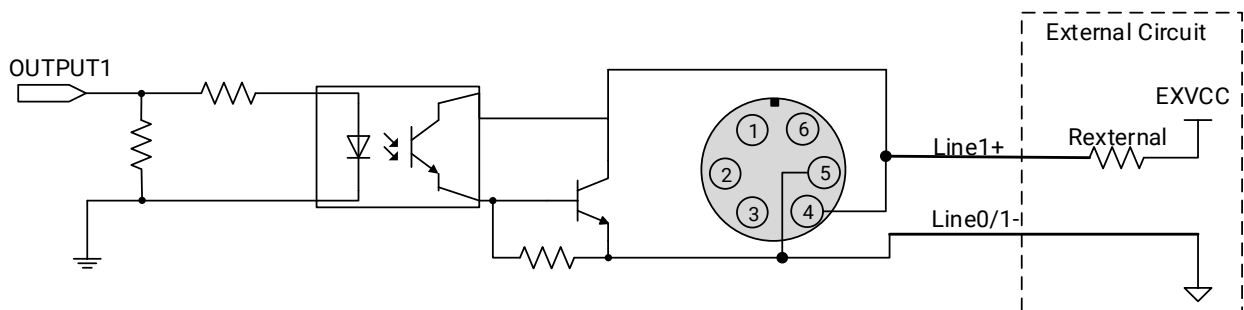
Figure 7-13 Opto-isolated output circuit (ME2S/ME2C)
