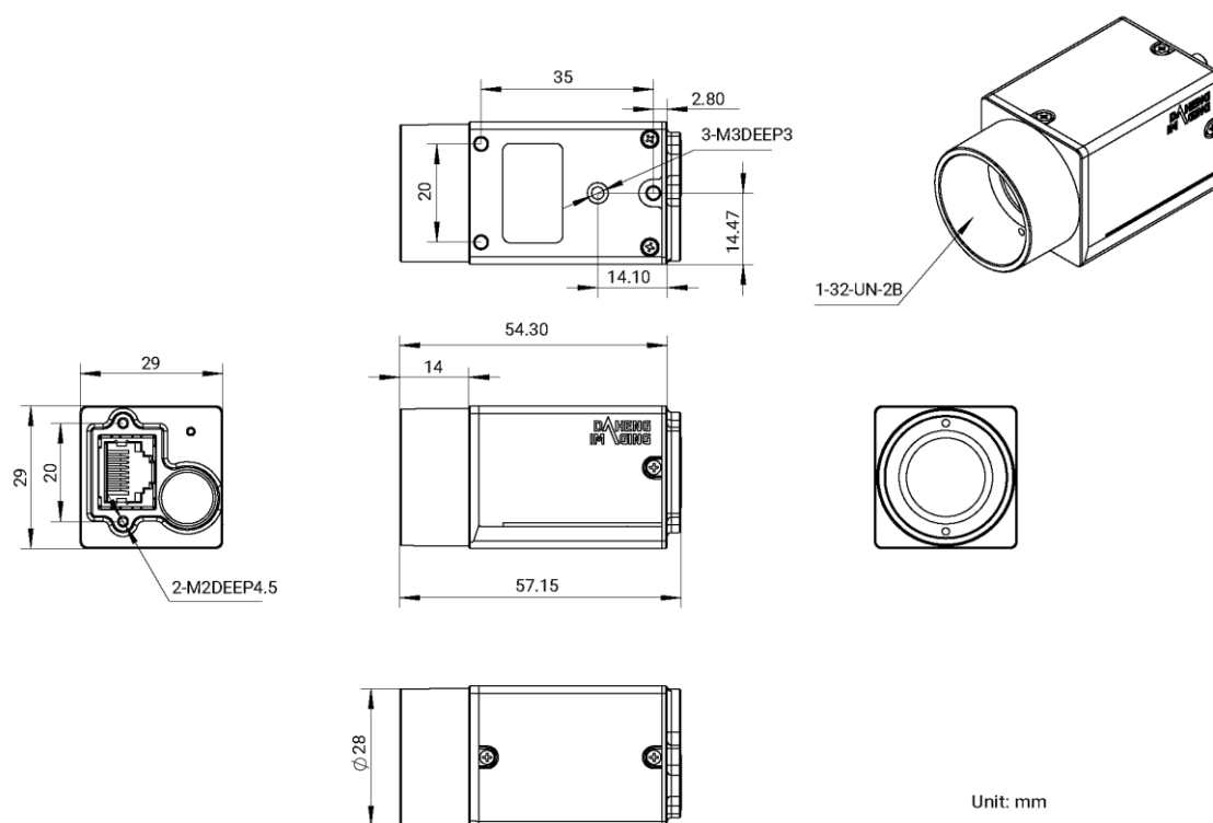
Figure 5-8 ME2C-G-P-L mechanical dimensions
