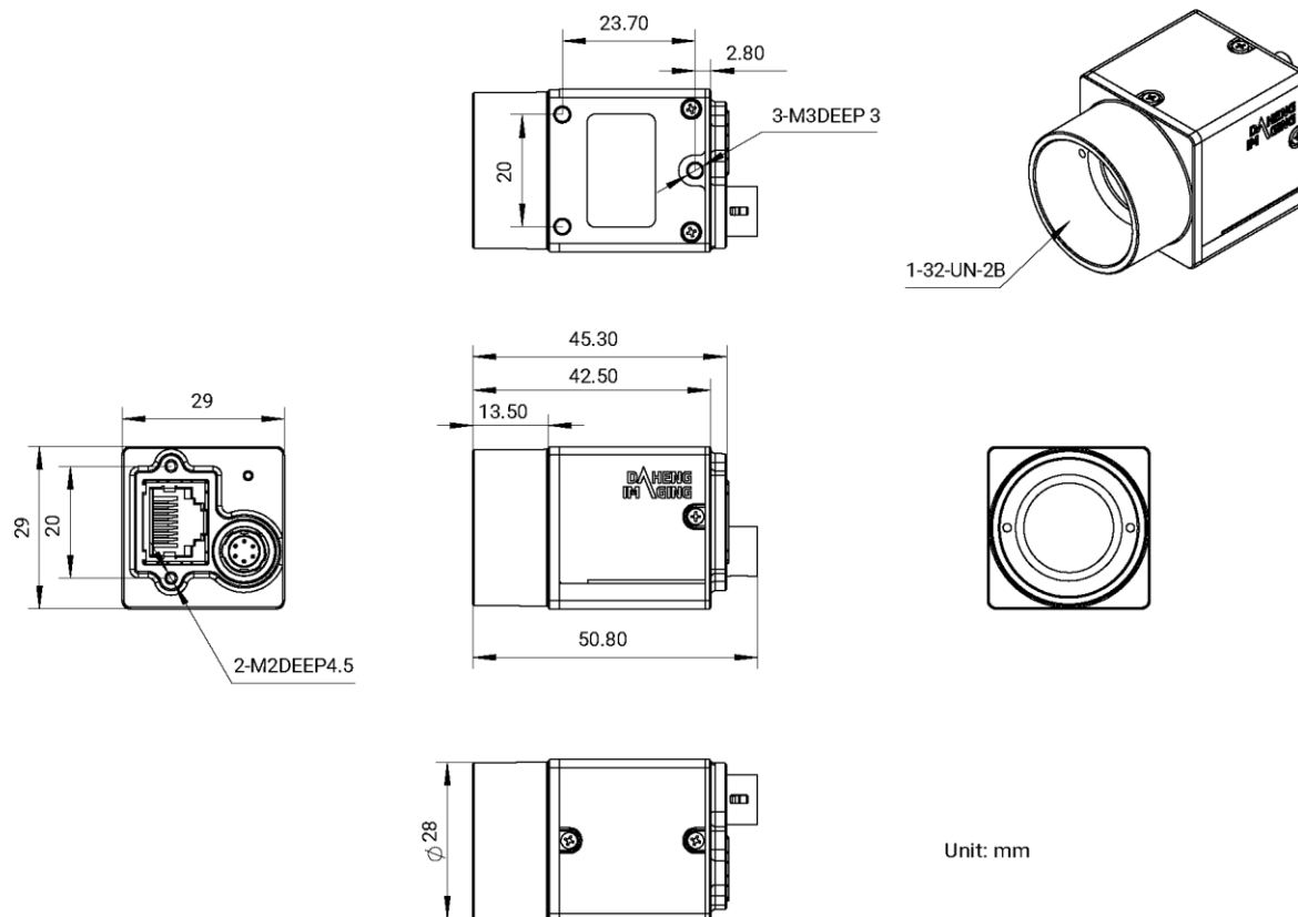
Figure 5-9 ME2C-051-120GM/C mechanical dimensions
