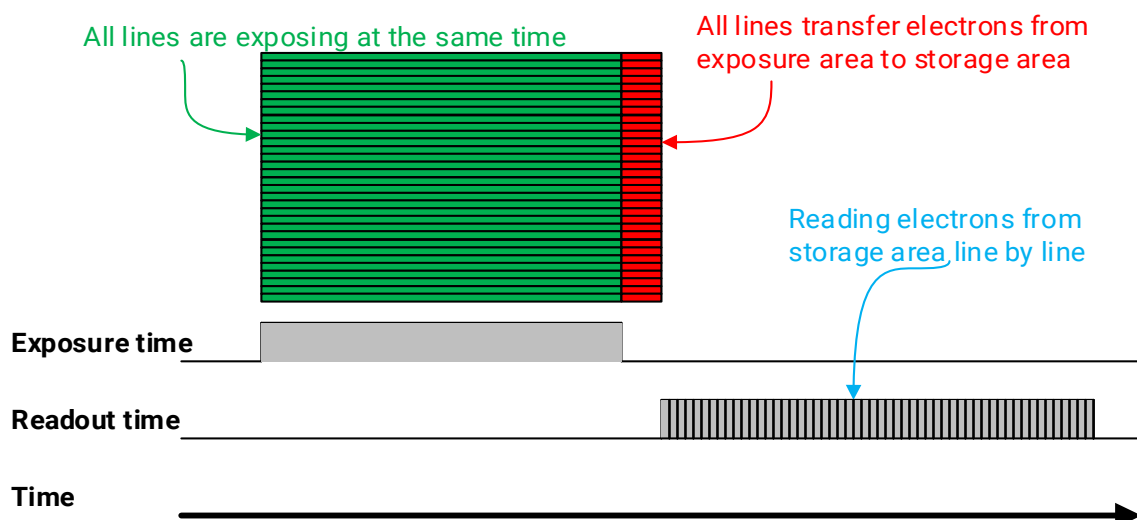
Figure 8-31 Global Shutter
