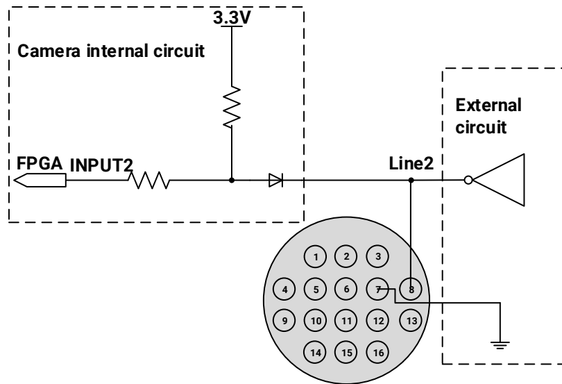
Figure 7-19 Internal equivalent circuit of camera when Line2 is configured as input (ME2P Multispectral)
