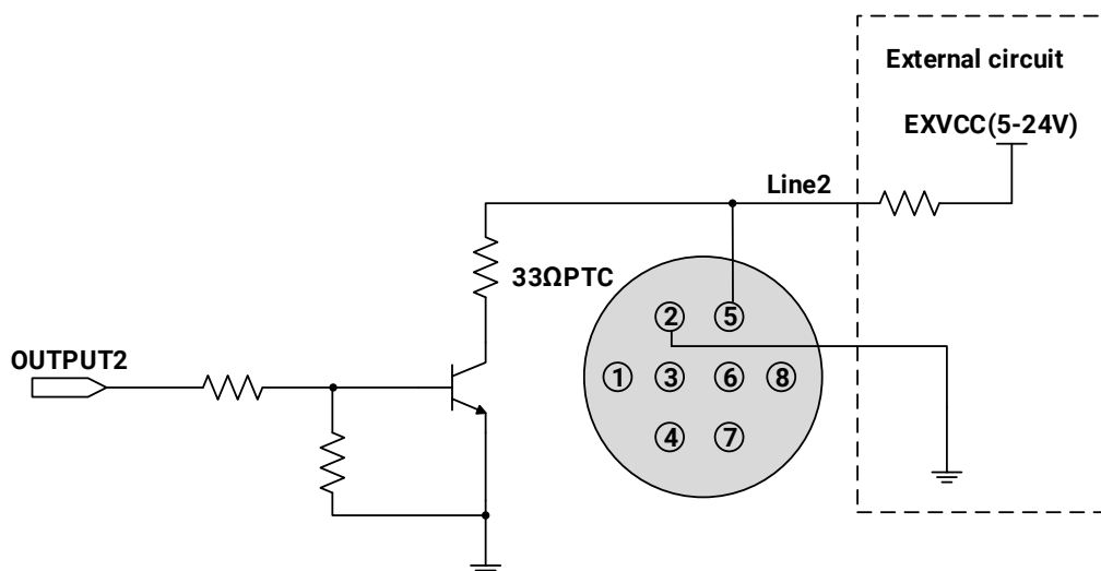
Figure 7-29 Internal equivalent circuit of camera when Line2 is configured as output (MER2/ME2P)
