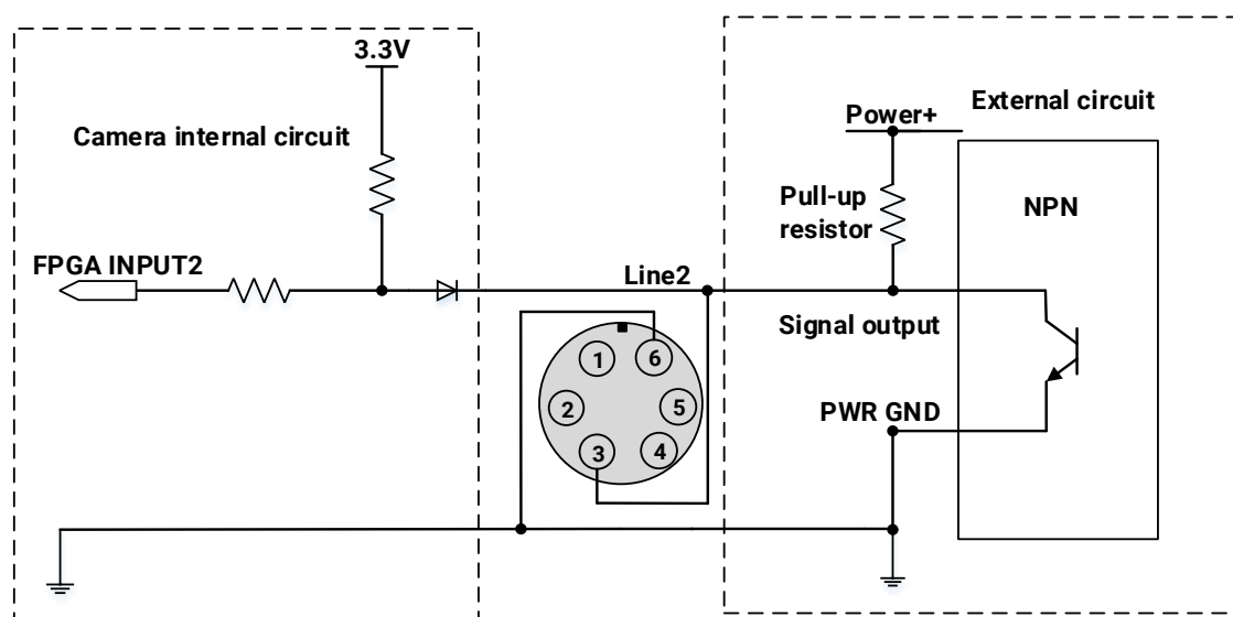
Figure 7-25 NPN photoelectric sensor connected to Line2 input circuit (ME2S/ME2C)
