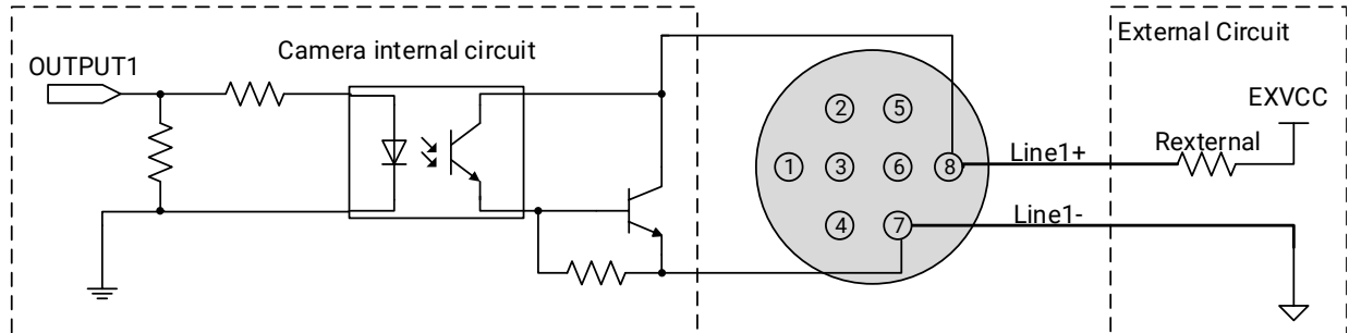
Figure 7-11 Opto-isolated output circuit (MER2/ME2P)
