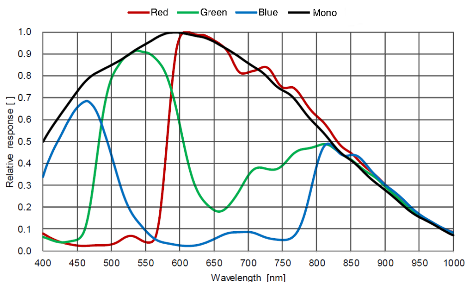
Figure 4-23 ME2C-042-121GM/C sensor spectral response
