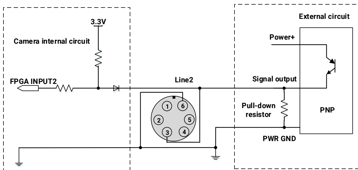
Figure 7-26 PNP photoelectric sensor connected to Line2 input circuit (ME2S/ME2C)
