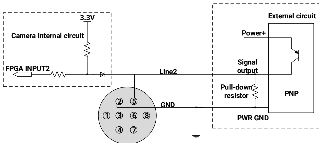
Figure 7-22 PNP photoelectric sensor connected to Line2 input circuit (MER2/ME2P)
