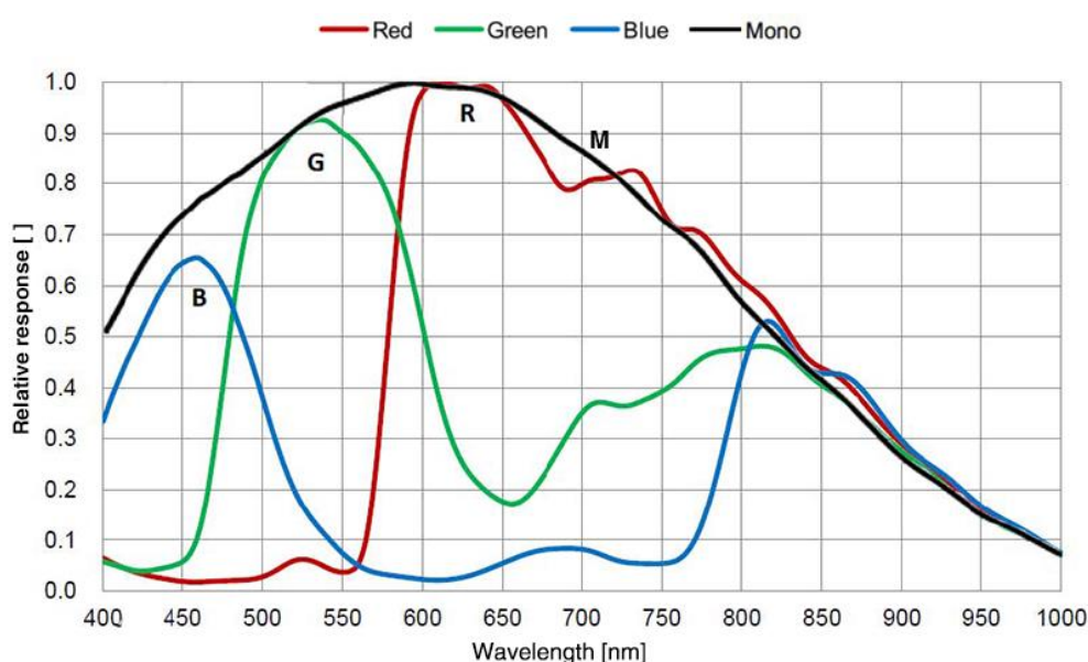
Figure 4-11 MER2-303-37GM/C(-P) sensor spectral response
