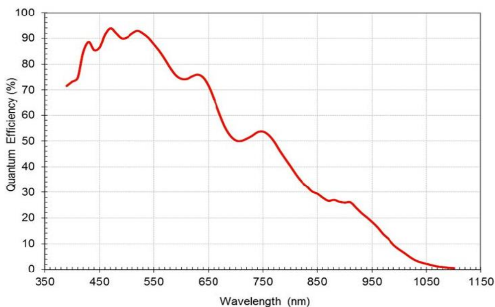
Figure 4-16 MER2-507-23GM(-P) NIR sensor spectral response
