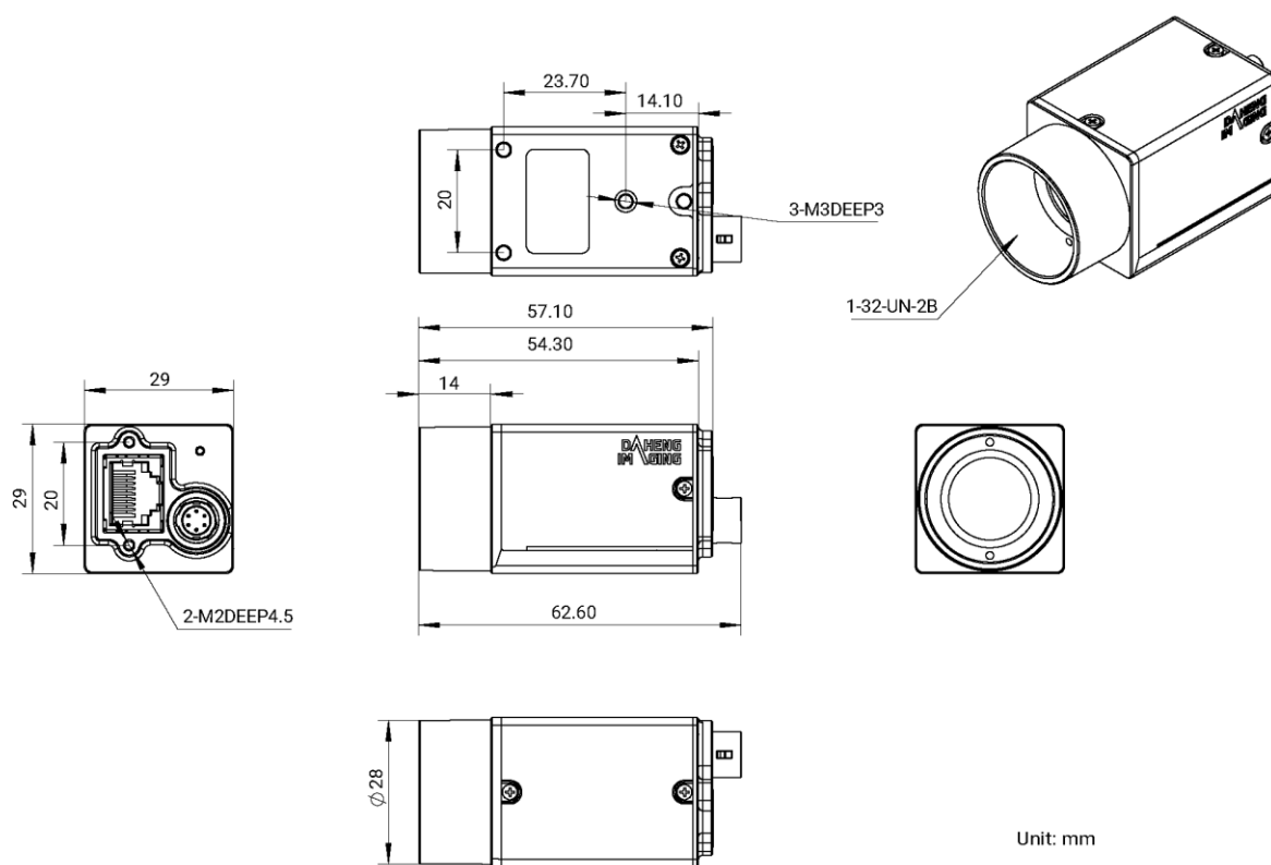
Figure 5-7 ME2C-G-P mechanical dimensions
