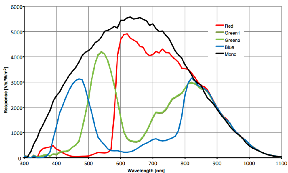
Figure 4-3 MER2-134-90GM/C(-P) sensor spectral response
