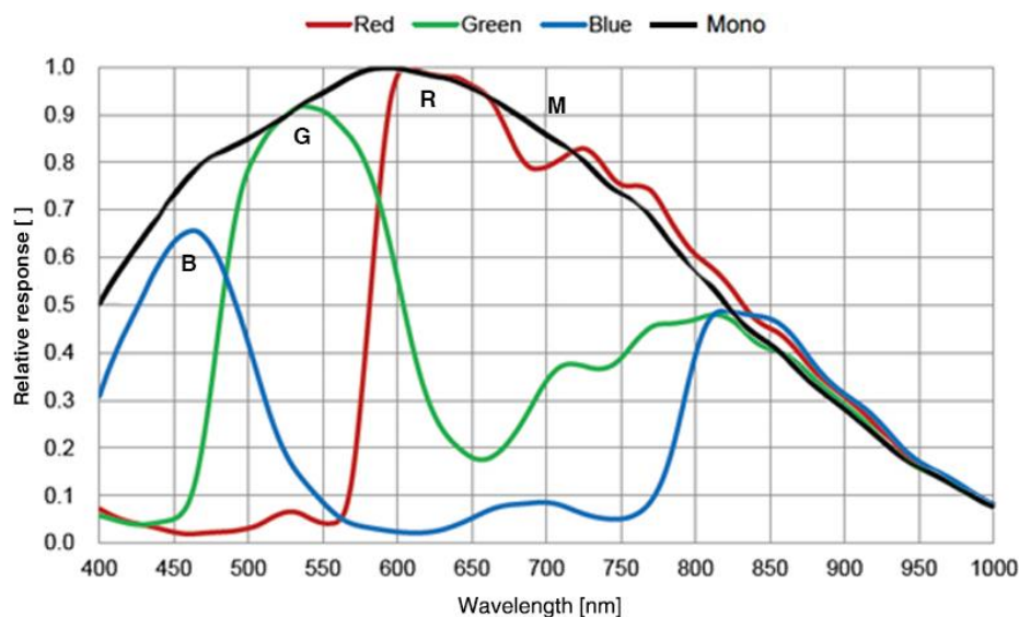
Figure 4-26 ME2C-160-75GM/C(-P) sensor spectral response
