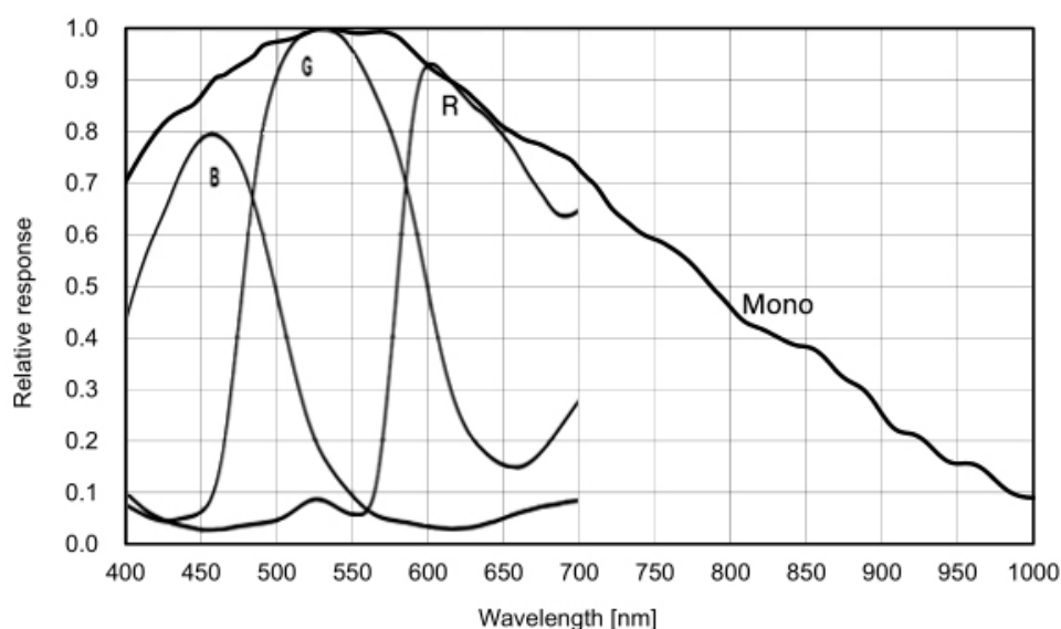
Figure 4-44 ME2C-2000-6GM/C(-P) sensor spectral response
