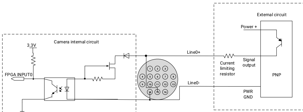
Figure 7-7 PNP photosensor connected to opto-isolated input circuit (ME2P Multispectral)
