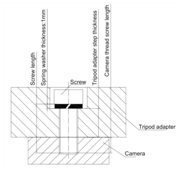
Figure 5-17 Schematic diagram of screw specification, tripod adapter step thickness and spring washer thickness
