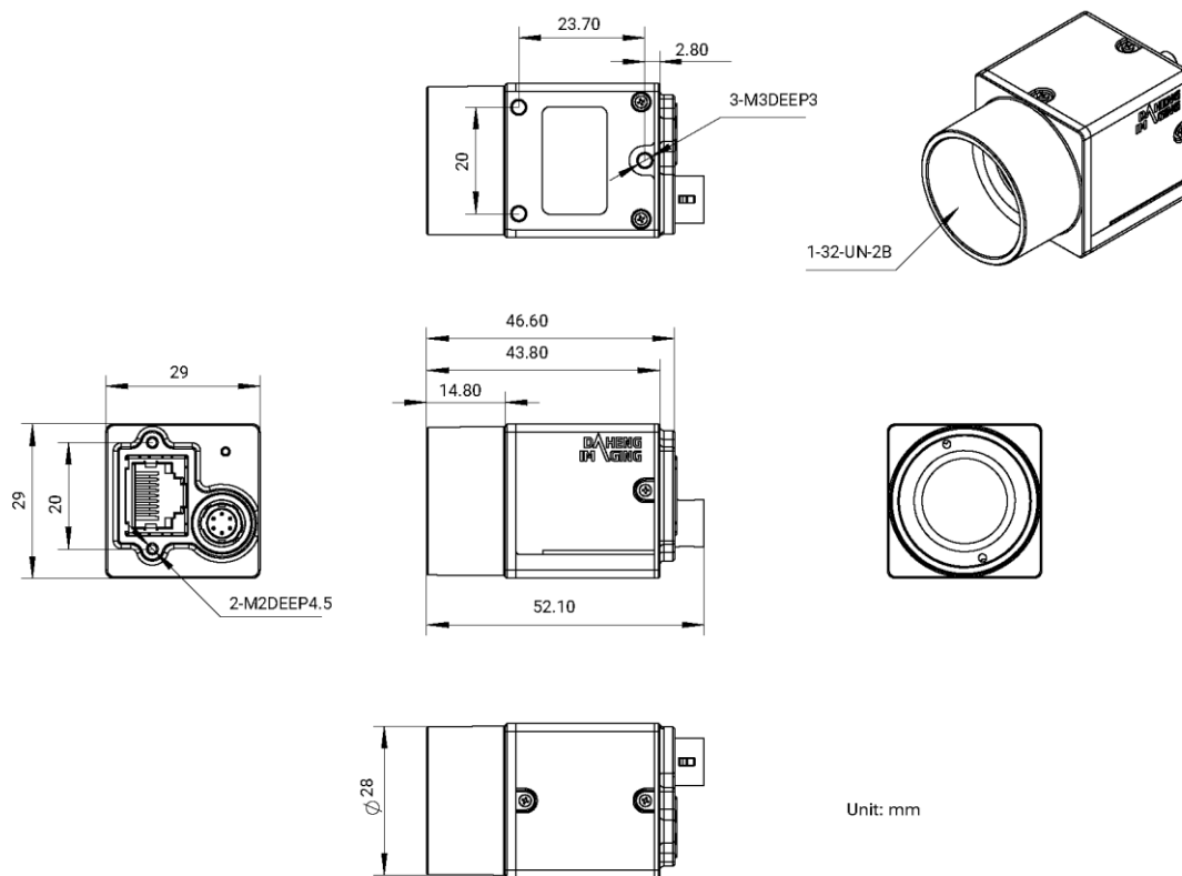
Figure 5-11 ME2C-532-22GM/C mechanical dimensions
