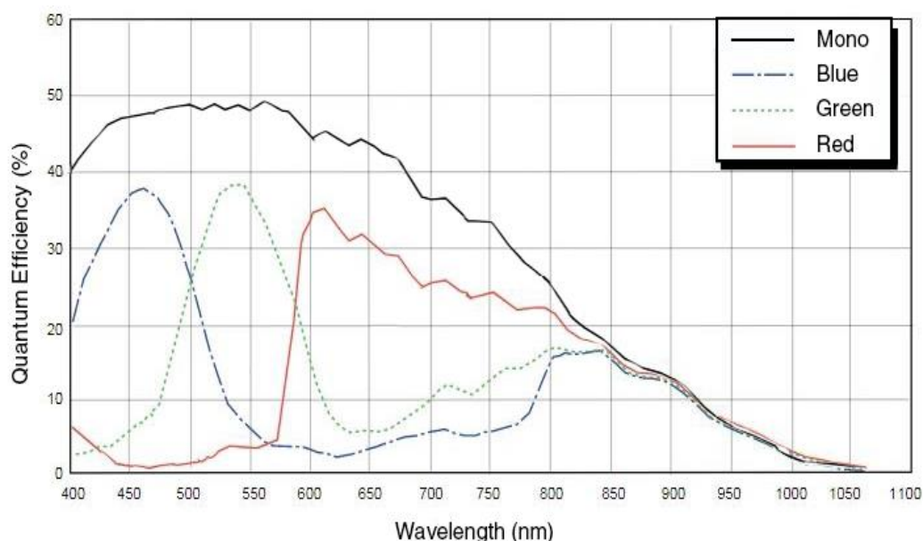
Figure 4-6 MER2-202-60GM/C(-P) sensor spectral response
