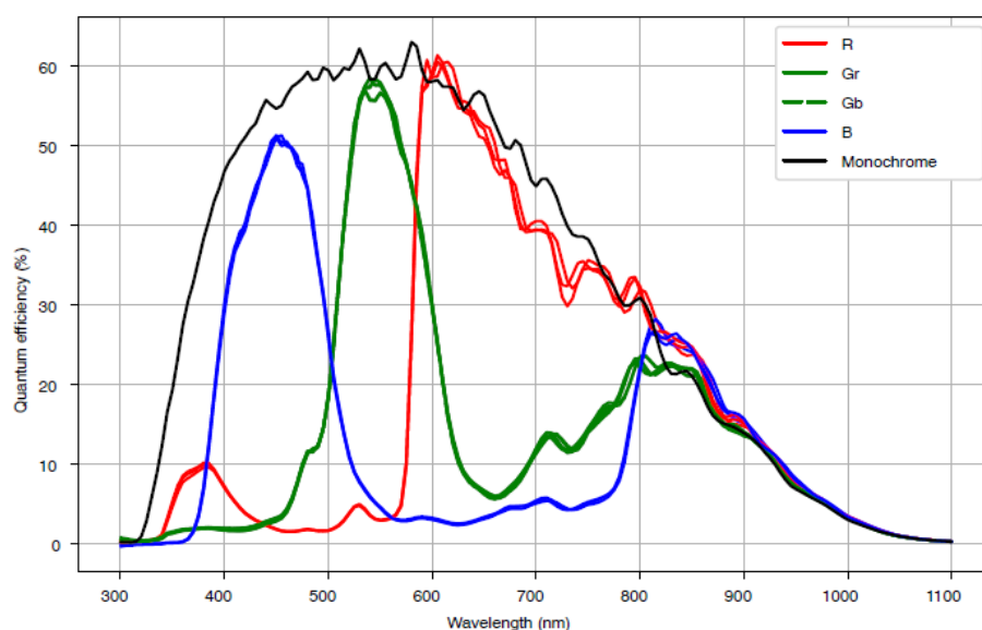
Figure 4-40 ME2C-532-22GM/C sensor spectral response
