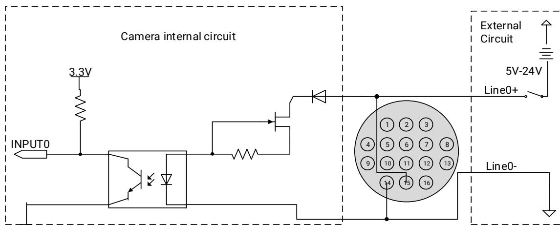
Figure 7-2 Opto-isolated input circuit (ME2P Multispectral)
