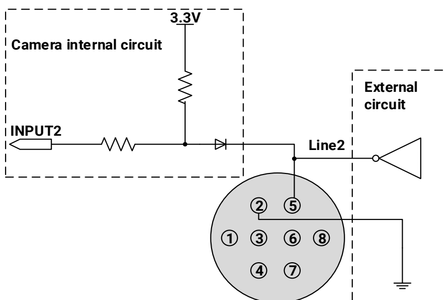
Figure 7-18 Internal equivalent circuit of camera when Line2 is configured as input (MER2/ME2P)
