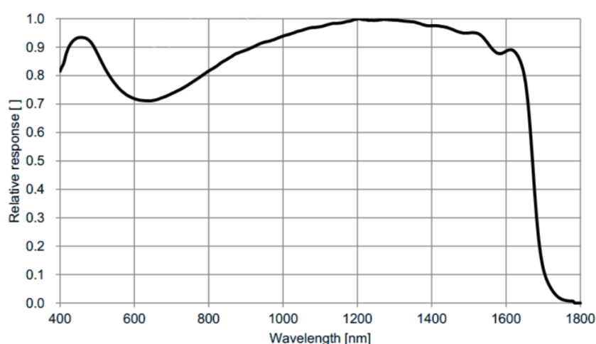
Figure 4-17 MER3-138-136G3M-P-SWIR sensor spectral response
