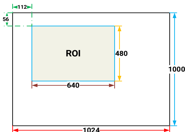
Figure 8-79 An example for the relative position between the ROI and the current image
