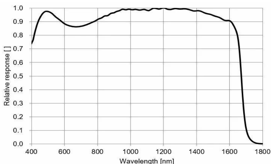
Figure 4-18 MER3-321-91G3M-P-SWIR sensor spectral response
