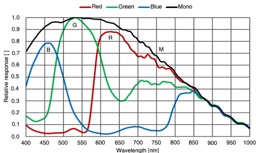
Figure 4-15 MER3-1221-24G3M/C-P-AF sensor spectral response
