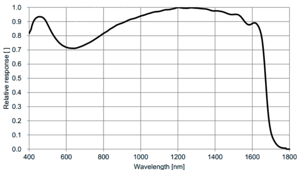
Figure 4-16 MER3-033-262G3M-P-SWIR sensor spectral response
