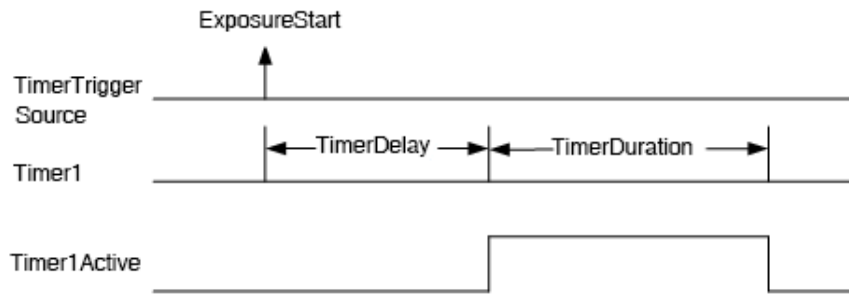
Figure 8-63 The schematic diagram of Timer1Active
