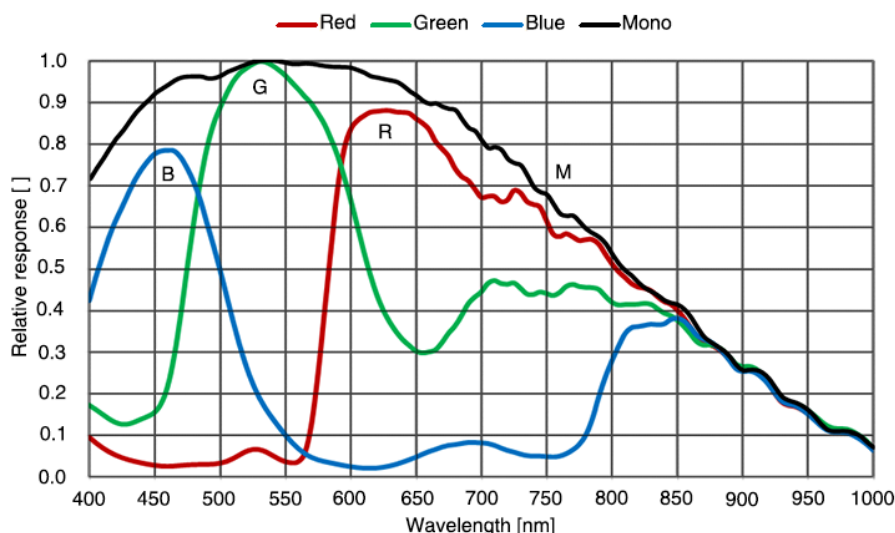
Figure 4-14 MER3-506-58G3M/C-P-AF sensor spectral response
