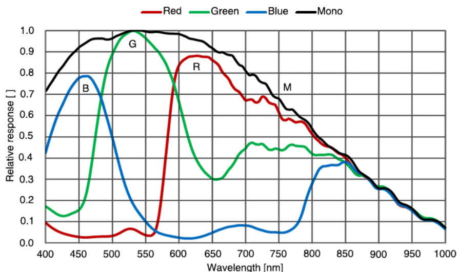
Figure 4-4 MER3-506-58G3M/C-P sensor spectral response
