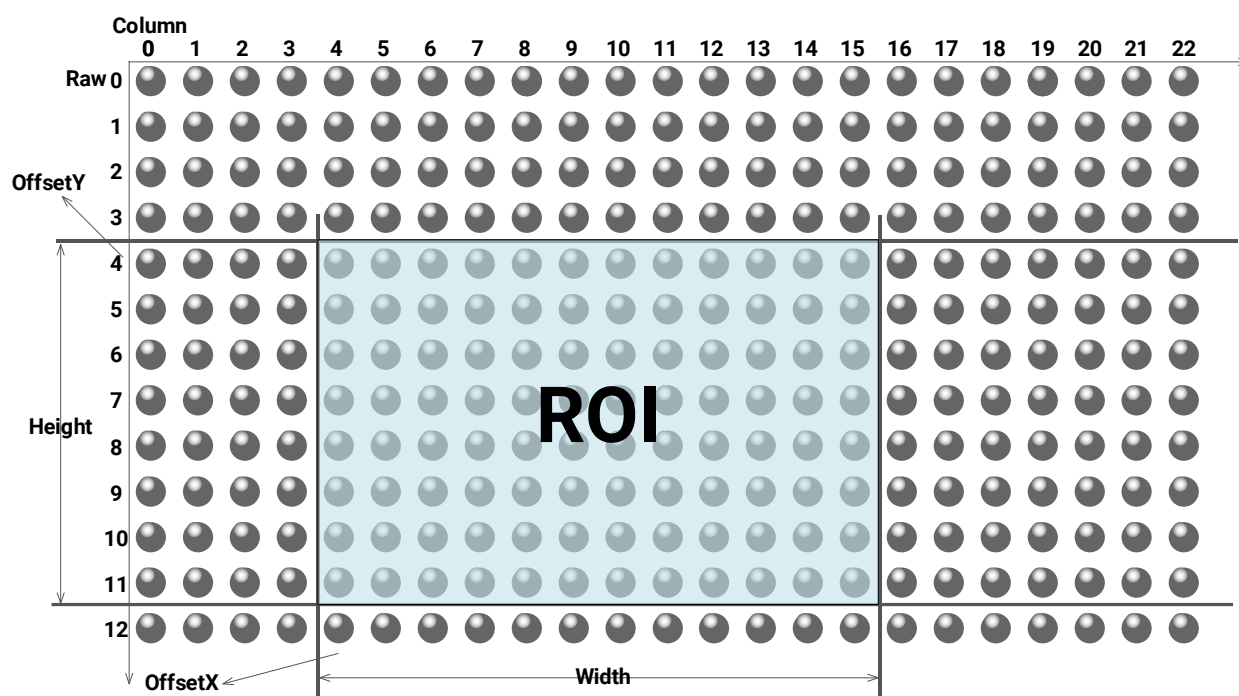
Figure 8-39 Mono8
