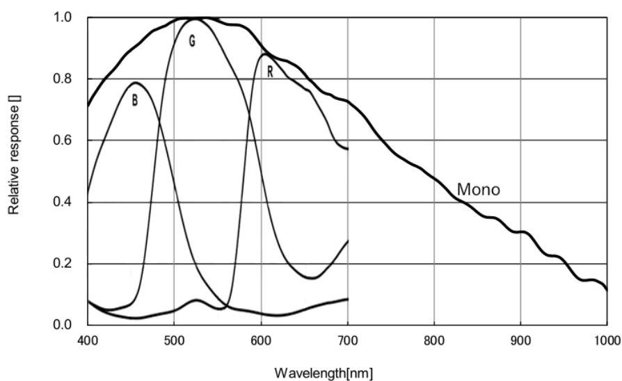
Figure 4-7 MER3-1220-24G3M/C-P sensor spectral response
