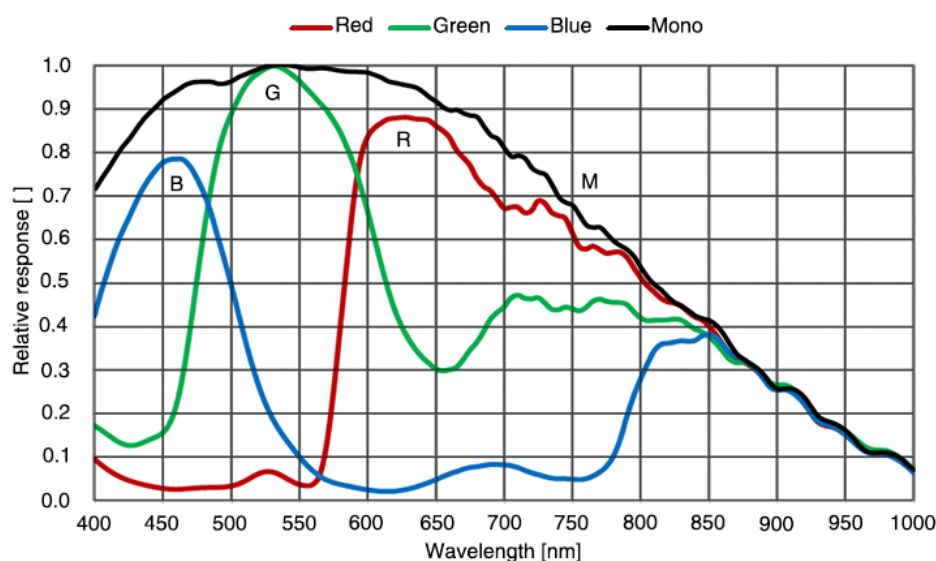
Figure 4-5 MER3-517-58G3M/C-P sensor spectral response
