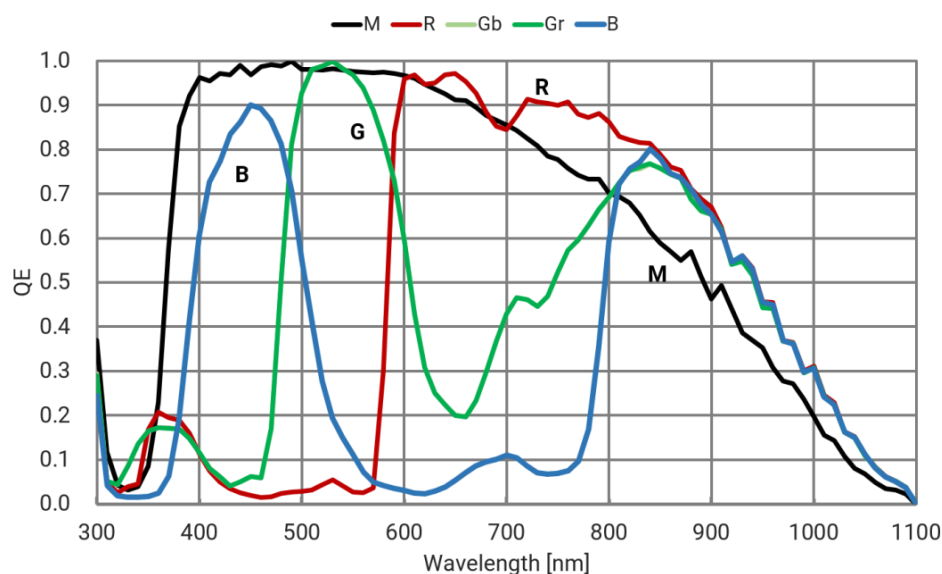
Figure 4-2 MER3-310-92G3M/C-P sensor spectral response
