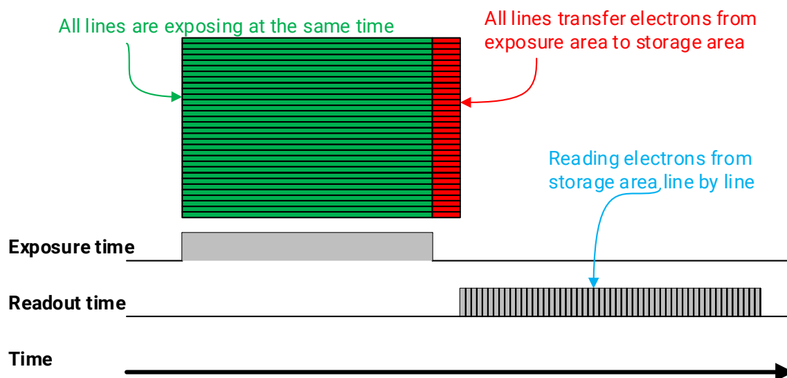
Figure 8-31 Global Shutter
