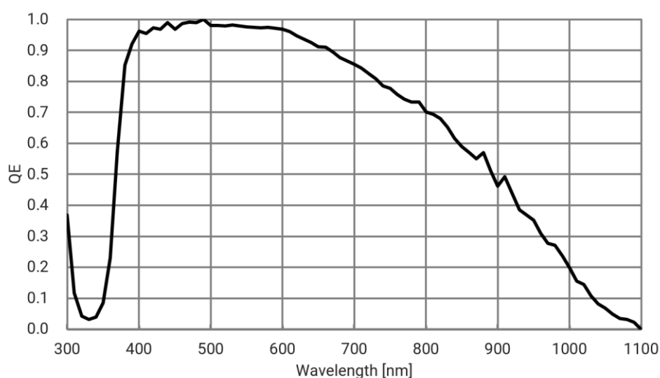
Figure 4-1 MER3-126-61G3M-P-NIR sensor spectral response
