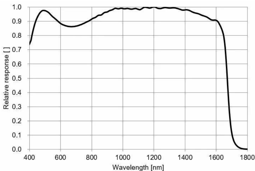
Figure 4-19 MER3-533-55G3M-P-SWIR sensor spectral response
