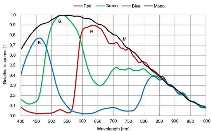
Figure 4-9 MER3-1610-18G3M/C-P sensor spectral response
