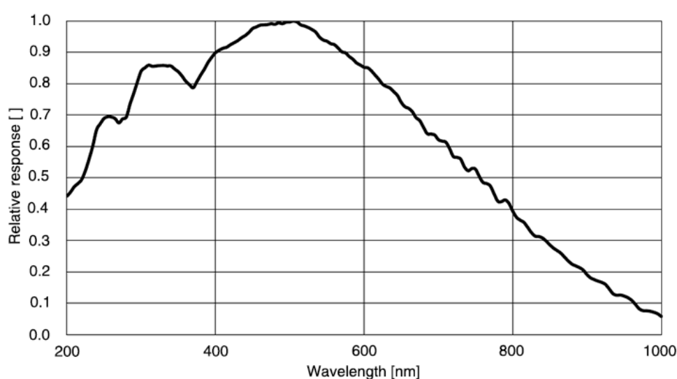
Figure 4-20 MER3-810-36G3M-P-UV sensor spectral response*
