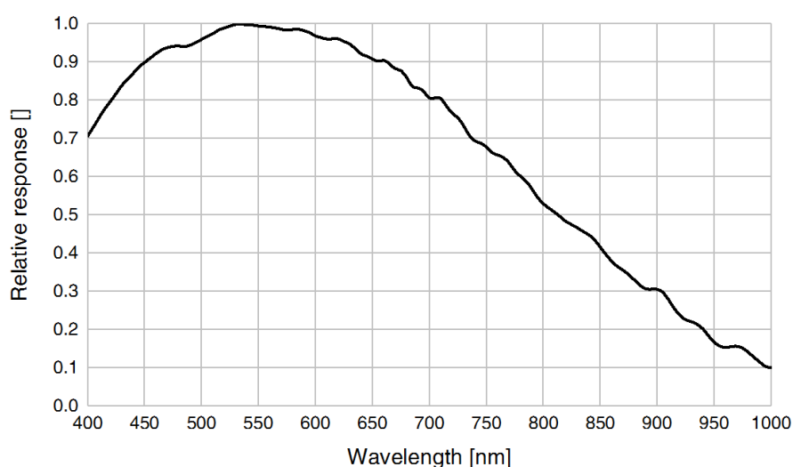
Figure 4-13 MER3-2560-11G3M-P sensor spectral response
