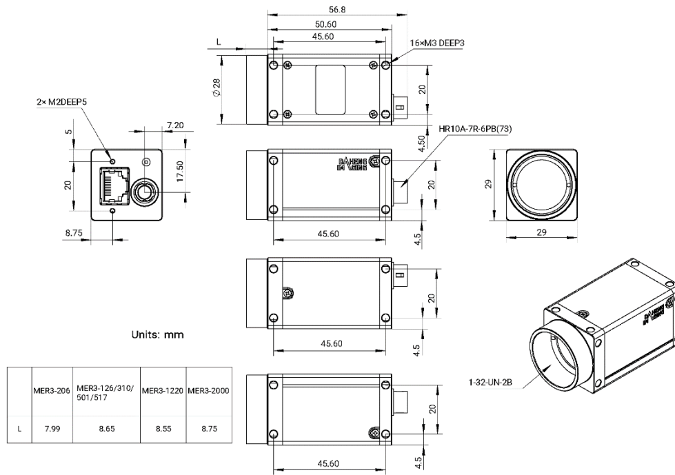
Figure 5-3 MER3-G3-P mechanical dimensions
