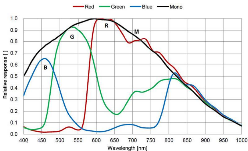
Figure 4-3 MER3-501-59G3M/C-P sensor spectral response
