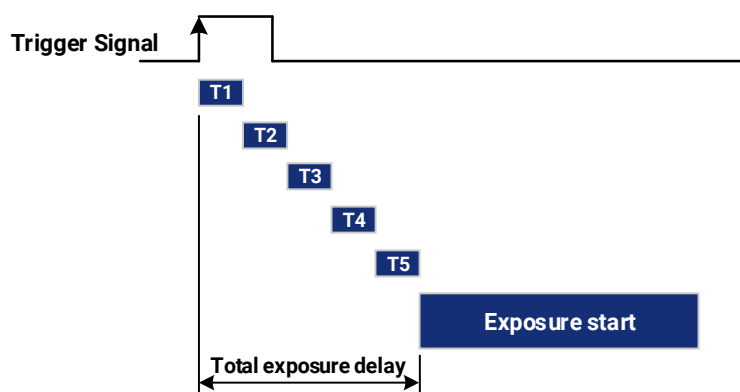
Figure 8-33 Exposure delay
