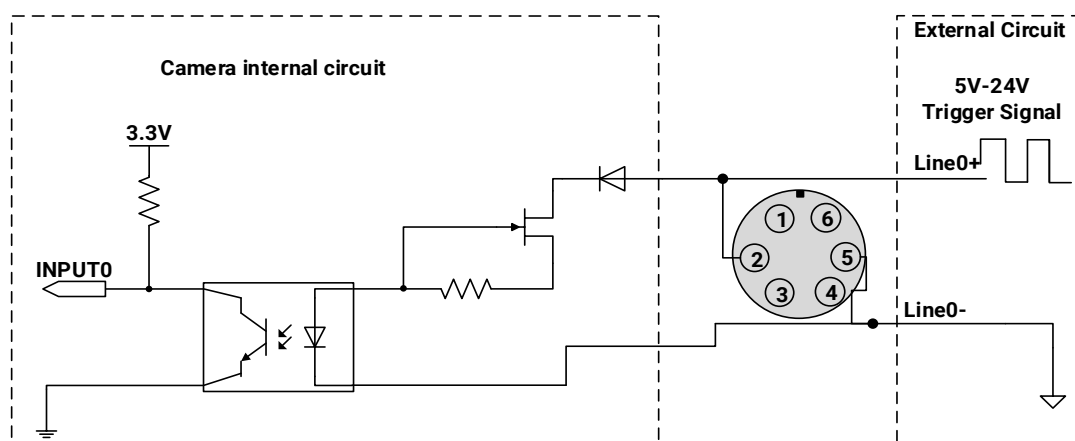
Figure 7-1 Opto-isolated input circuit
