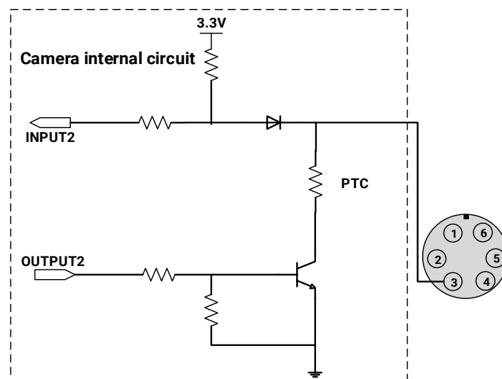
Figure 7-5 Line2 (bidirectional) circuit
