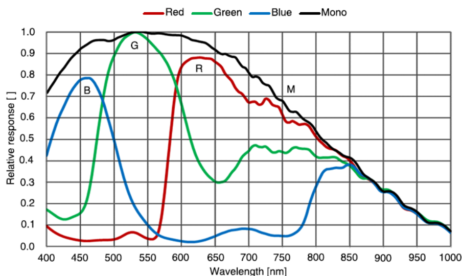
Figure 4-6 MER3-800-36G3M/C-P sensor spectral response
