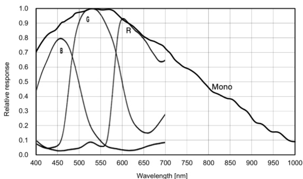
Figure 4-10 MER3-2000-15G3M/C-P sensor spectral response
