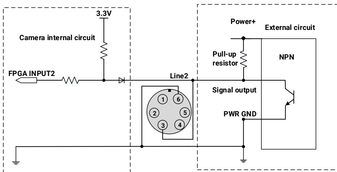
Figure 7-7 NPN photoelectric sensor connected to Line2 input circuit
