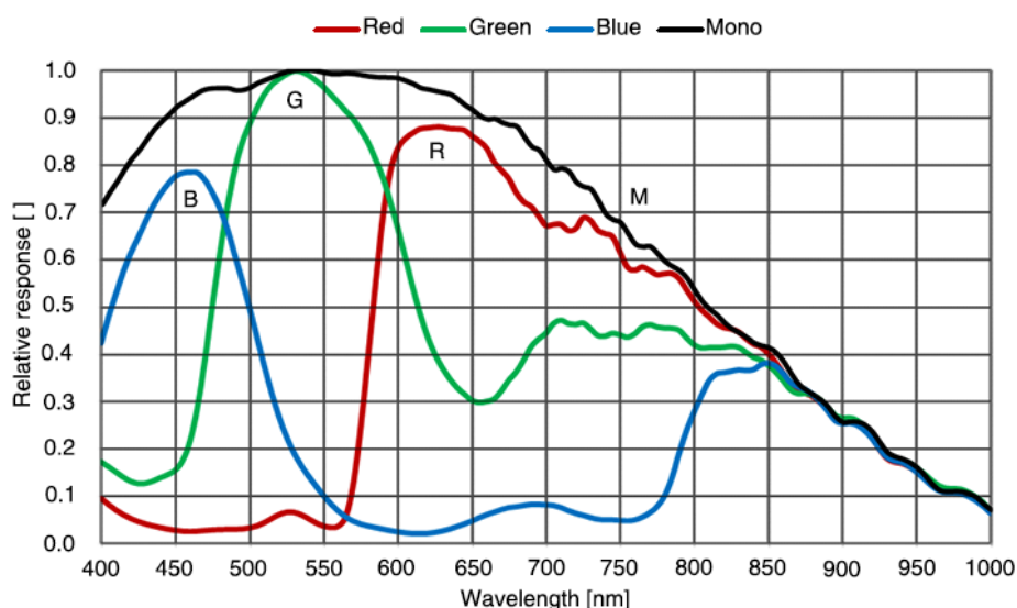
Figure 4-8 MER3-1221-24G3M/C-P sensor spectral response
