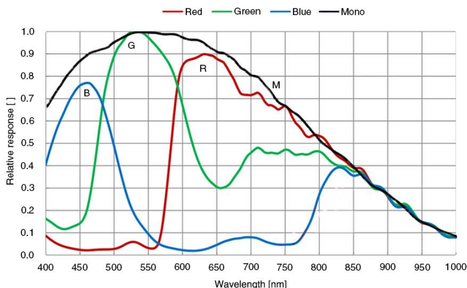
Figure 4-12 MER3-2440-12G3M/C-P sensor spectral response
